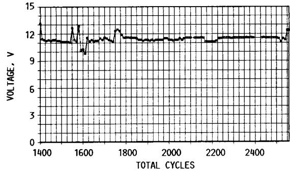
FIGURE 5. - DISCHARGE KEEPER VOLTAGE.
