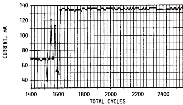
FIGURE 4. - DISCHARGE KEEPER CURRENT.
