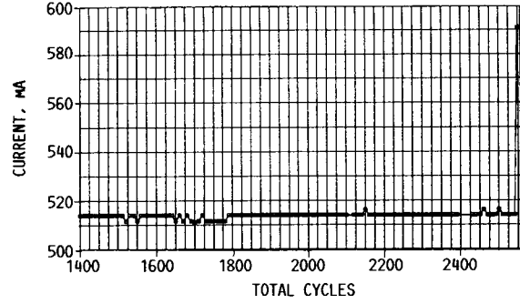
FIGURE 12. - NEUTRALIZER KEEPER CURRENT.
