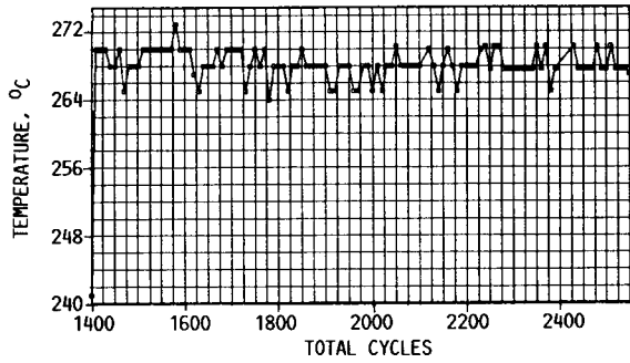
FIGURE 8. - DISCHARGE VAPORIZER TEMPERATURE.
