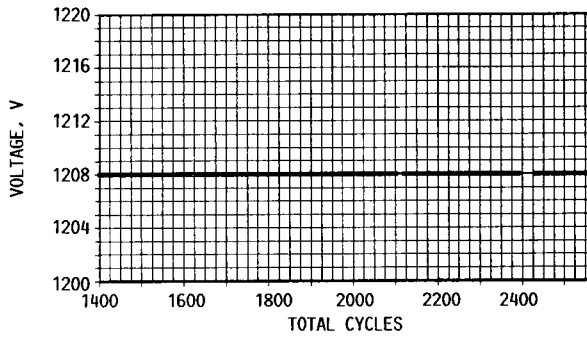
FIGURE 3. - SCREEN VOLTAGE.
