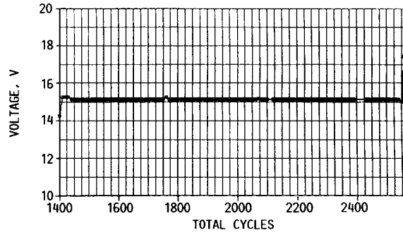
FIGURE 13. - NEUTRALIZER KEEPER VOLTAGE.
