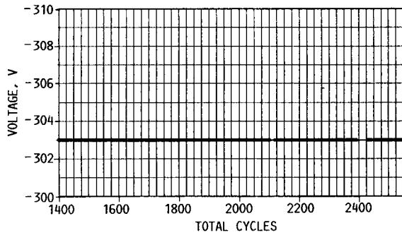
FIGURE 10. - ACCELERATOR VOLTAGE.
