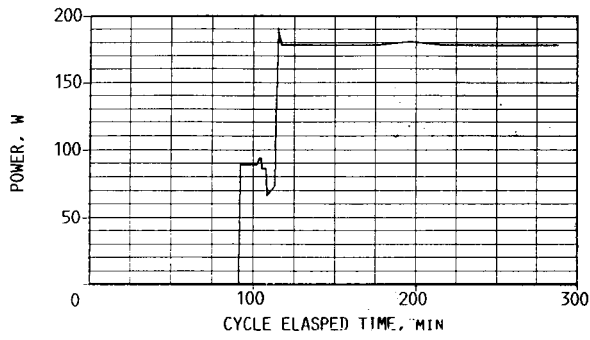
FIGURE 16. - TOTAL POWER CONSUMED.
