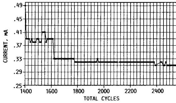
FIGURE 9. - ACCELERATOR CURRENT.
