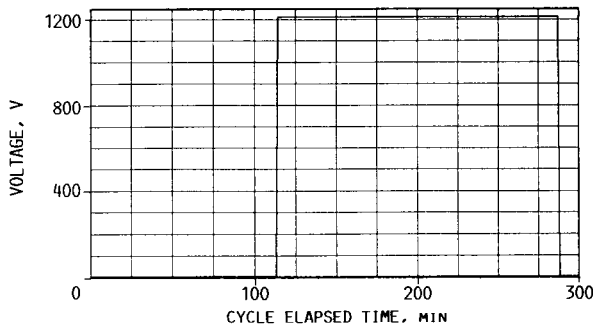
FIGURE 18. - SCREEN VOLTAGE.
