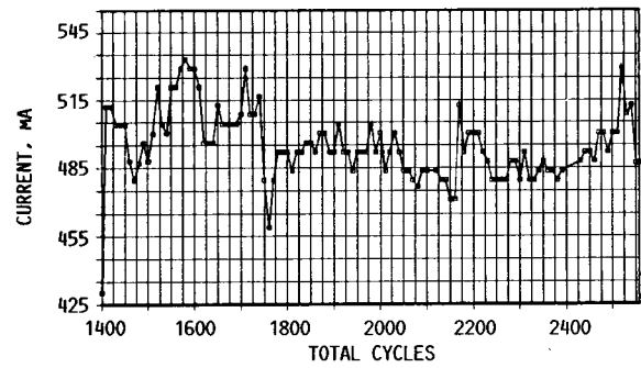
FIGURE 6. - DISCHARGE CURRENT.
