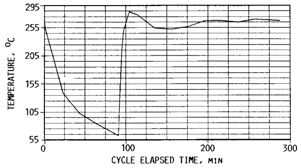
FIGURE 19. - DISCHARGE VAPORIZER TEMPERATURE.
