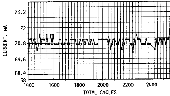
FIGURE 2. - SCREEN CURRENT.
