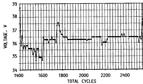
FIGURE 7. - DISCHARGE VOLTAGE.
