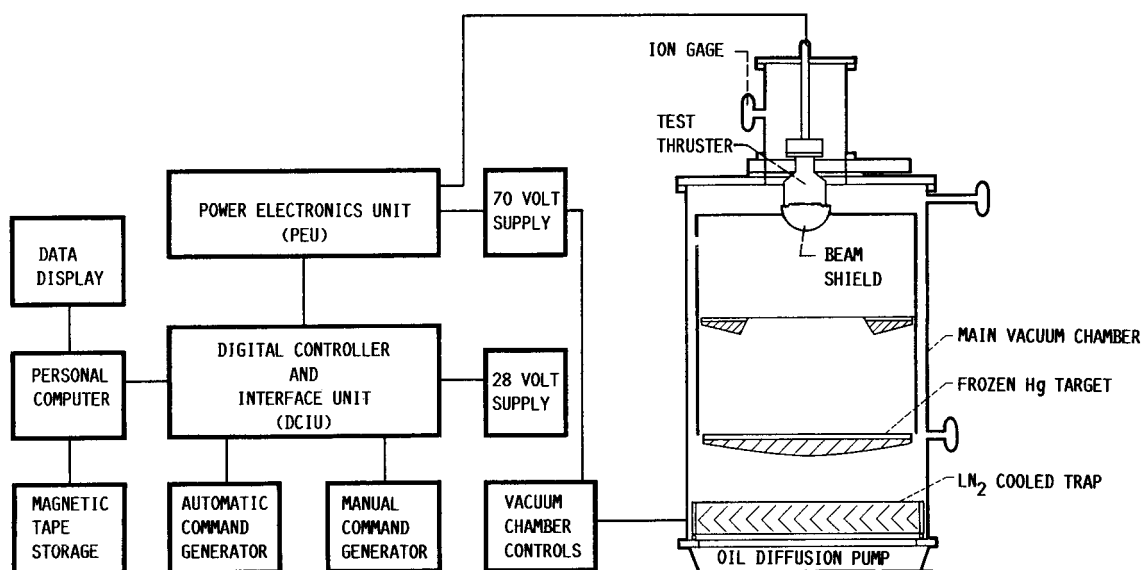
FIGURE 1. - GROUND TEST FACILITY AND ELECTRONICS BLOCK DIAGRAM.
