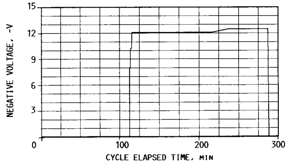
FIGURE 21. - NEUTRALIZER FLOATING POINT POTENTIAL.
