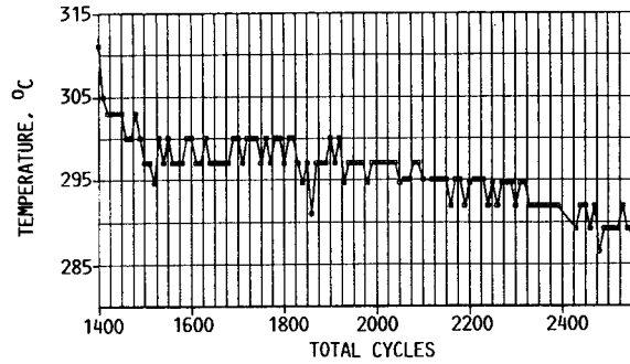
FIGURE 14. - NEUTRALIZER VAPORIZER TEMPERATURE.
