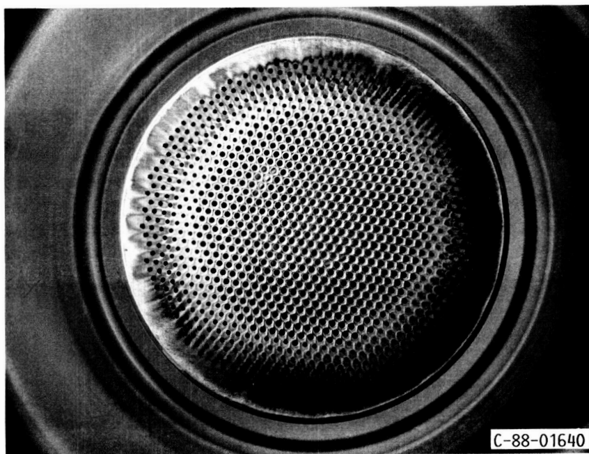
FIGURE 24. - POST TEST ACCELERATOR GRID.
