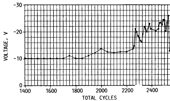
FIGURE 11. - NEUTRALIZER FLOATING POINT POTENTIAL.
