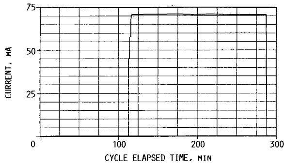
FIGURE 17. - SCREEN CURRENT.
