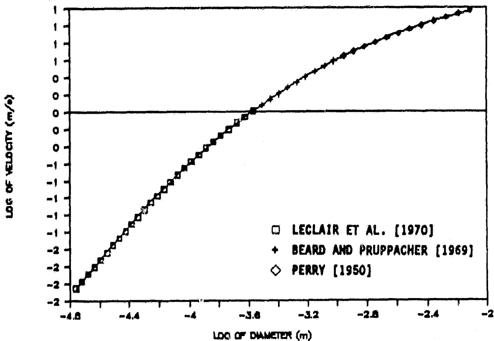
Figure 2. Comparison of the sedimentation velocity in the absence of an electric field for spherical particles given by Equation (16) with those given by LeClair et al. [1970], Beard and Pruppacher [1969], and Perry [1950], p = 1000 \text{ mb} , \Delta\rho = 1000 \text{ kg/m}^3 .
