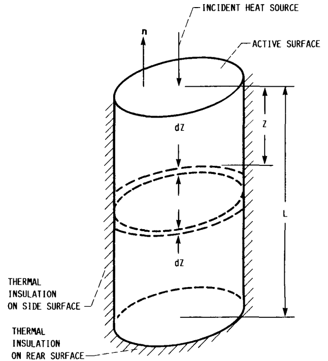
Figure 2.—Heat balance on thermoplug.
