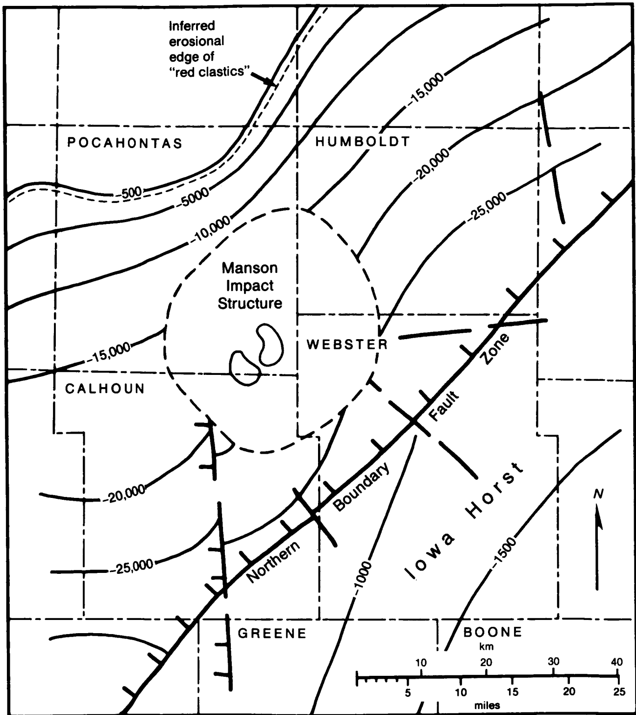
Fig. 4. Map showing elevation from sea level of the top of the Precambrian crystalline surface in the area of the Manson Impact Structure as determined by gravity modeling. Elevations are in feet and contour intervals are variable.
