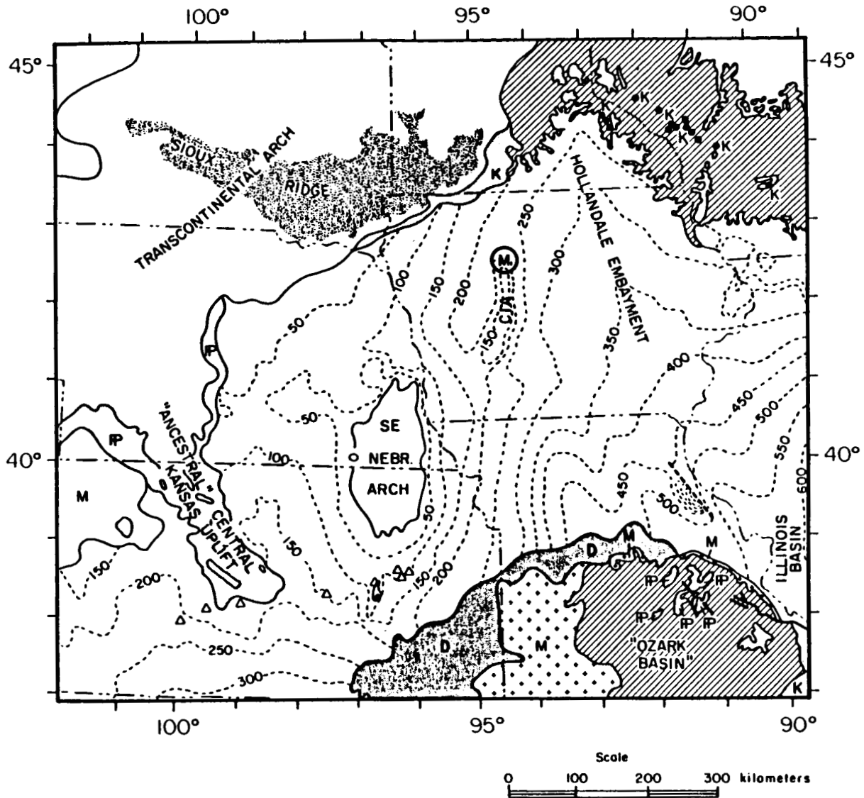
Fig. 7. Isopach map of Sauk sequence rocks (Cambrian to Lower Ordovician) in the central midcontinent (modified from Bunker et al. , in press, Fig. 2). The location of the Manson Impact Structure is indicated by M and the Central Iowa Arch by CIA. The contour interval is 50 m.
