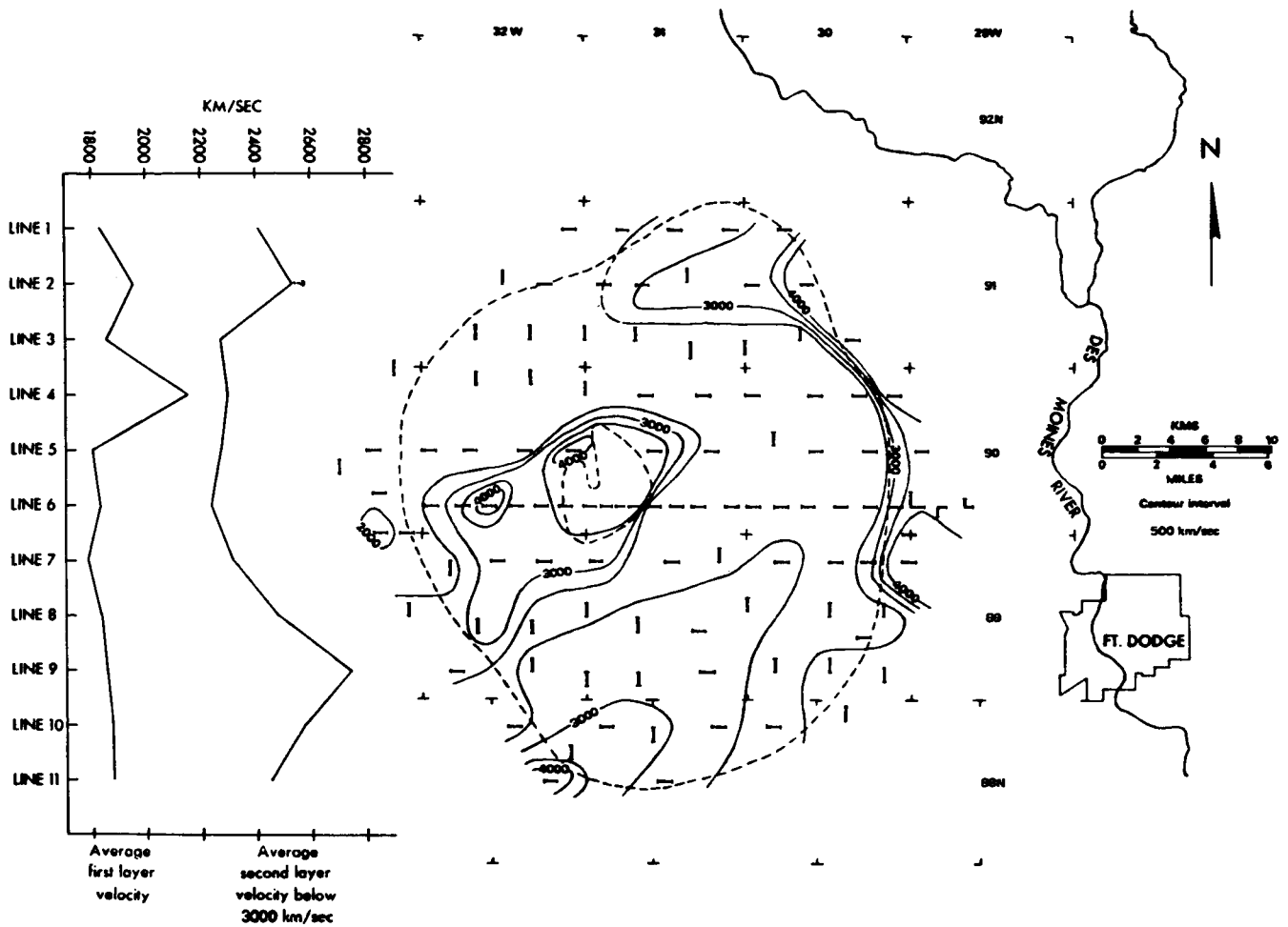
Fig. 23. Seismic wave propagation velocities in layers 1 and 2 averaged for 11 east-west lines and map of the area around Manson, Iowa, showing locations of geophone lines and contours of equal seismic velocity from Smith (1971), roughly concentric dashed lines indicate boundaries of "disturbed" area and the central "peak" of granitic bedrock, from Hershey (1969).
