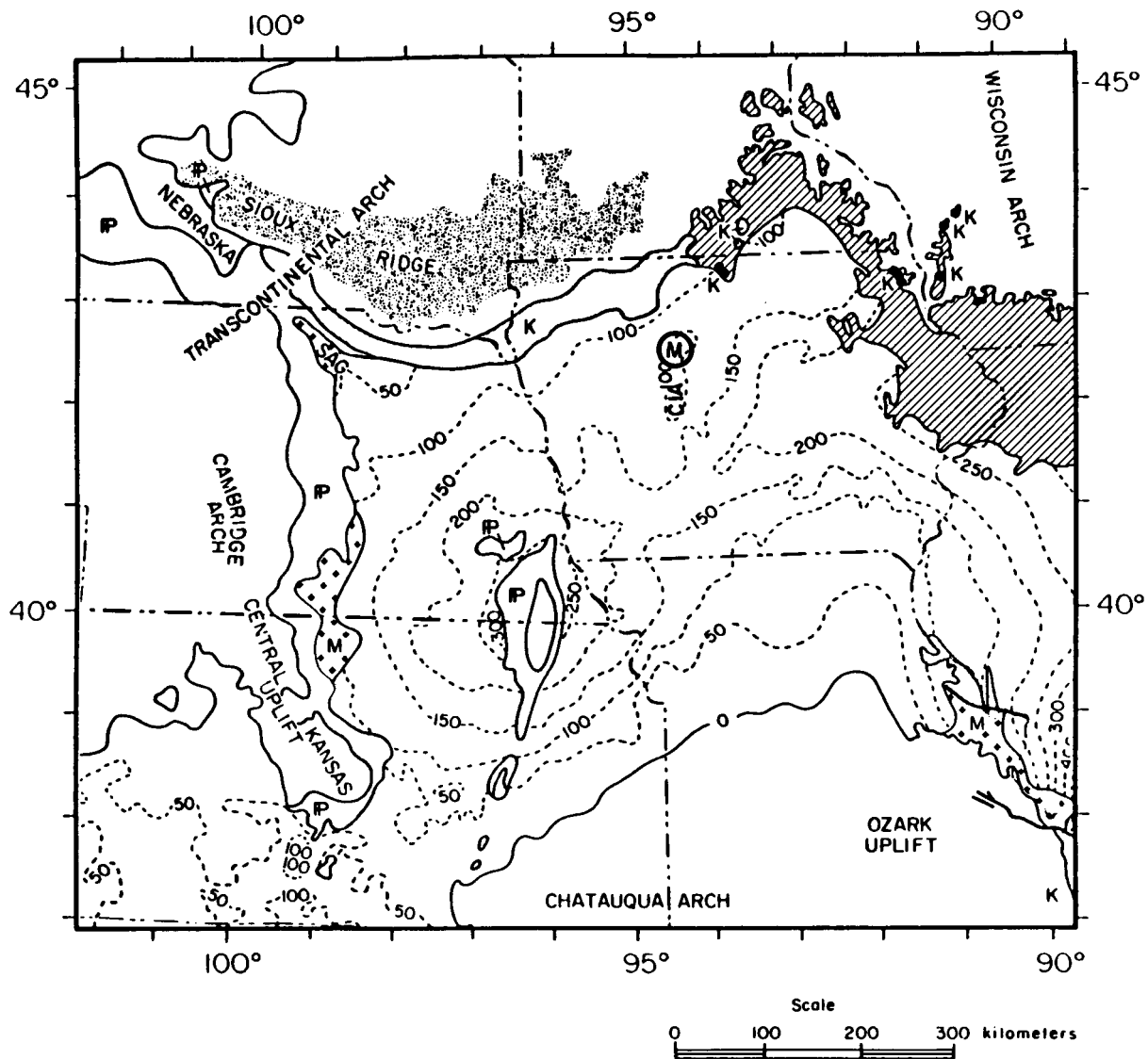
Fig. 8. Isopach map of Tippecanoe sequence rocks (Middle Ordovician-to-Silurian) in the central midcontinent (modified from Bunker et al. , in press, Fig. 3). The location of the Manson Impact Structure is indicated by M, and the Central Iowa Arch by CIA. The contour interval is 50 m.
