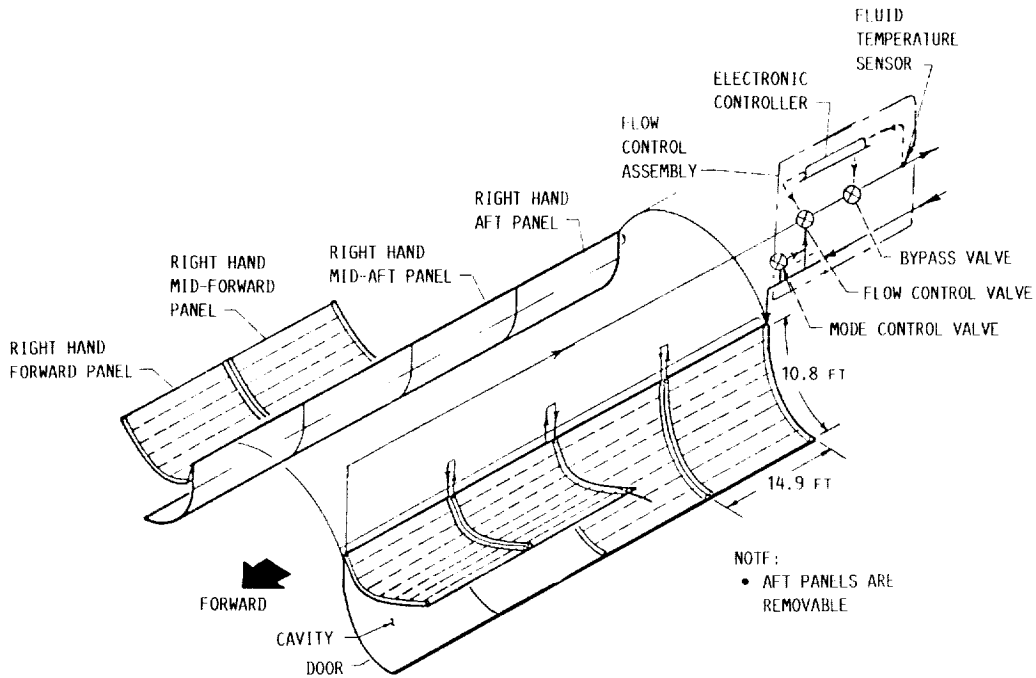
FIGURE 6. - ORBITER RADIATOR FLOW SCHEMATIC.
