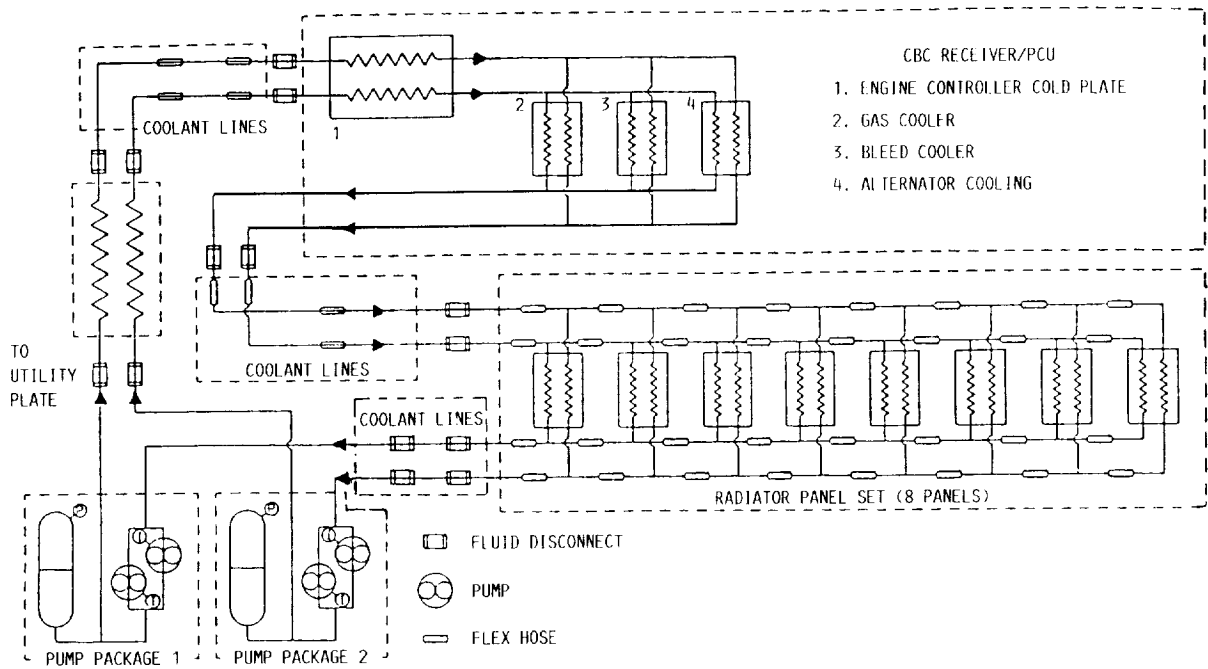
FIGURE 8. - SOLAR DYNAMIC RADIATOR PUMPED-FLUID LOOP FLOW SCHEMATIC.
