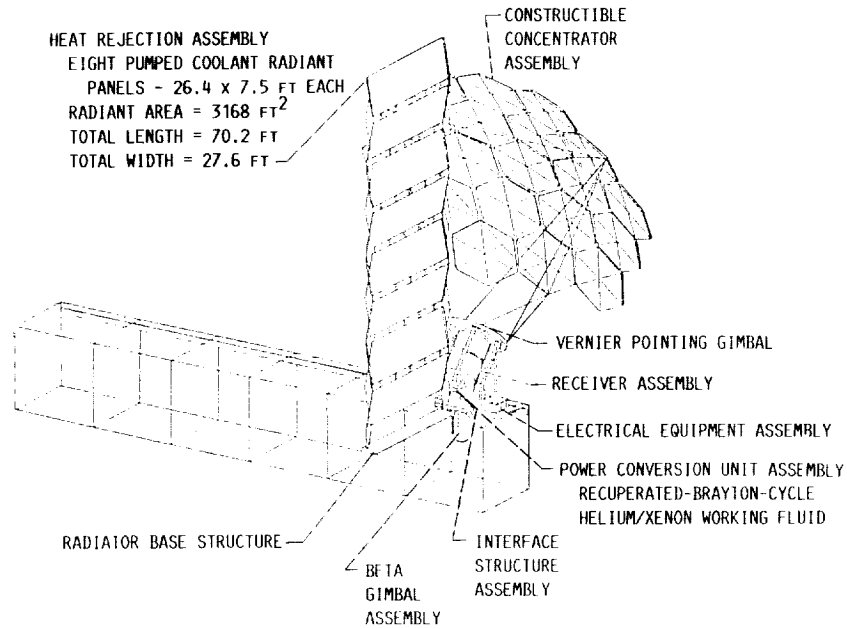
FIGURE 9. - THE SOLAR DYNAMIC POWER MODULE OPERATIONAL CONFIGURATION.
