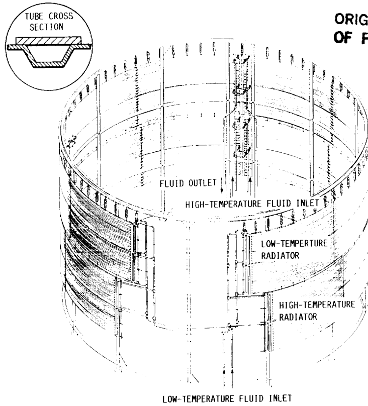
FIGURE 7. - THE BRAYTON ROTATING UNIT SPACE RADIATOR CONFIGURATION.
