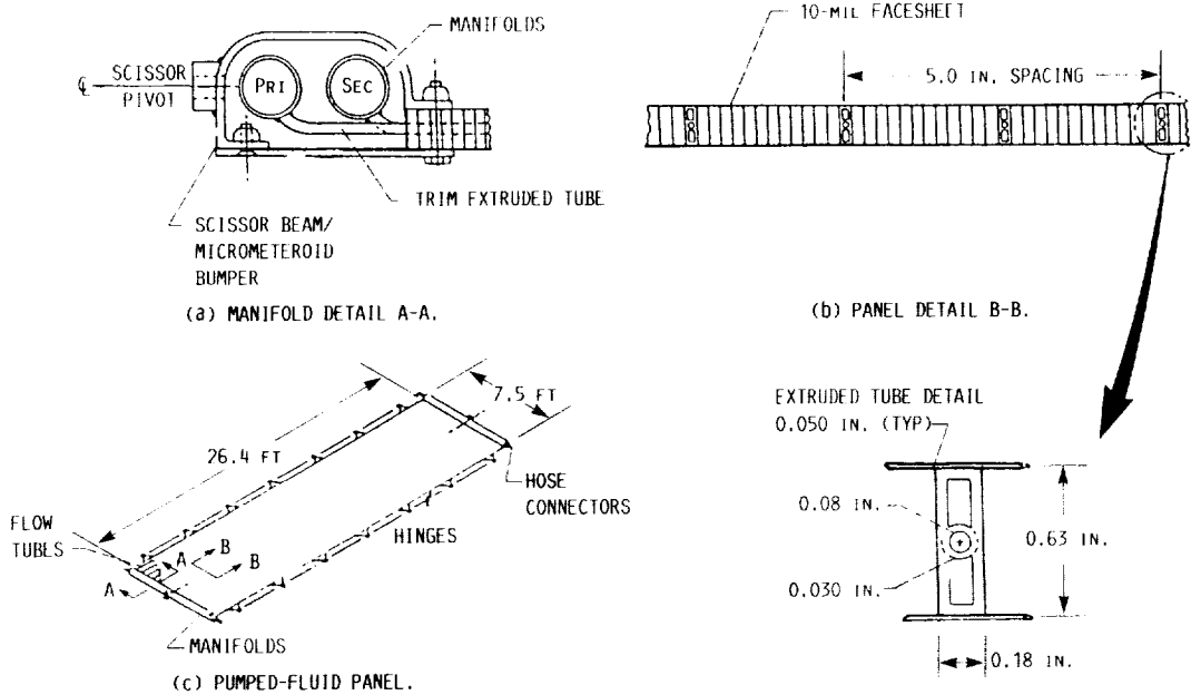
FIGURE 10. - SOLAR DYNAMIC RADIATOR PANEL STRUCTURE.
