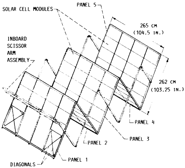
FIGURE 4. - THE ATM SOLAR ARRAY SCISSORS ARM DEPLOYMENT MECHANISM.
