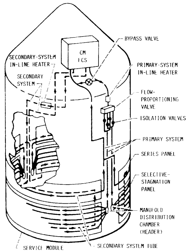
FIGURE 1. - SELECTIVE STAGNATION/FLOW PROPORTIONING RADIATOR SYSTEM FOR THE APOLLO CSM.
