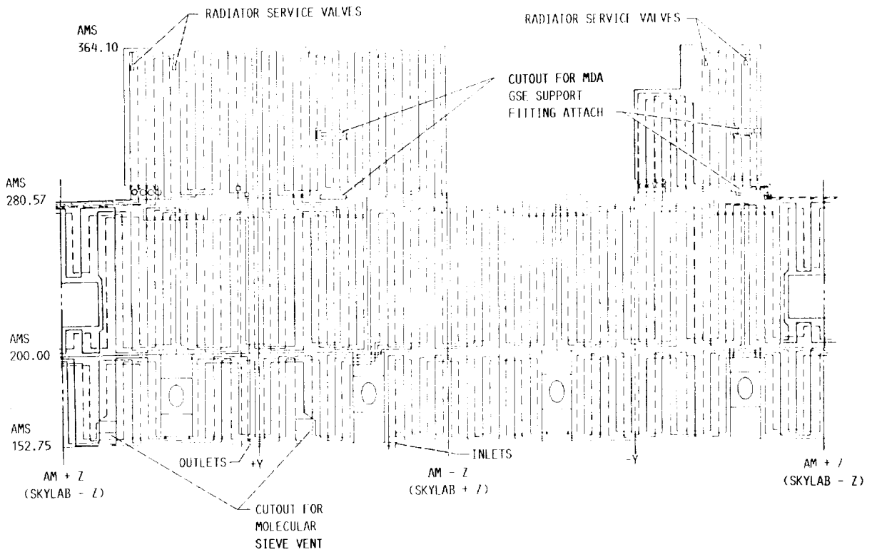
FIGURE 3. - THE AM/MDA RADIATOR STRETCHOUT LOOKING OUTBOARD.
