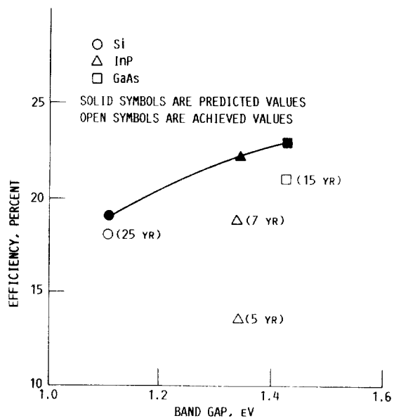
FIGURE 7. - PREDICTED AND ACHIEVED AMO EFFICIENCIES.
