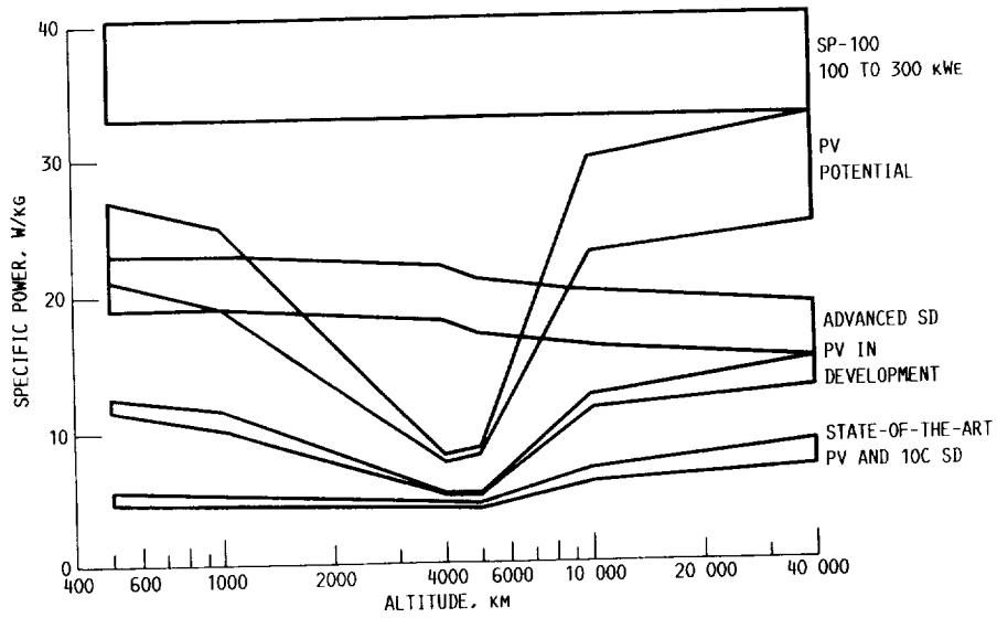
FIGURE 3. - SPECIFIC POWER COMPARISONS FOR SILICON PHOTOVOLTAIC SYSTEMS, ADVANCED SOLAR DYNAMIC AND NUCLEAR SYSTEMS, 5-YEAR LIFE.
