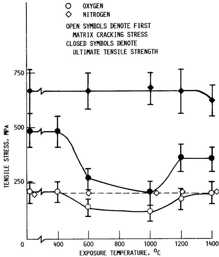
FIGURE 10. - ROOM TEMPERATURE TENSILE STRENGTHS FOR UNIDIRECTIONALLY REINFORCED sic/RBSN COMPOSITES ( v_f \sim 0.3 ) AFTER 100 HR EXPOSURE AT TEMPERATURES TO 1400 °C IN NITROGEN AND IN OXYGEN ENVIROMENTS.
