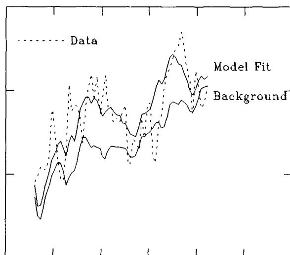
Fig. 3. Fit to data in the 1552–1624Å region.
