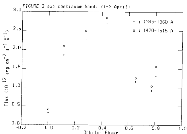
Figure 3. The continuum flux for 1-2 April 1987 in the regions 1345-1360 Å and 1470-1515 Å via orbital phase.
