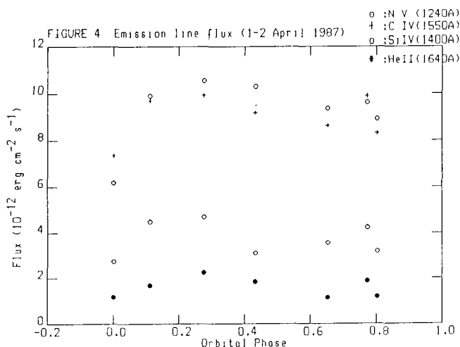
Figure 4. Variation of the Emission lines NV (1240 Å), Si IV (1400 Å), CIV (1550 Å), He II (1640 Å) on the orbital timescale
