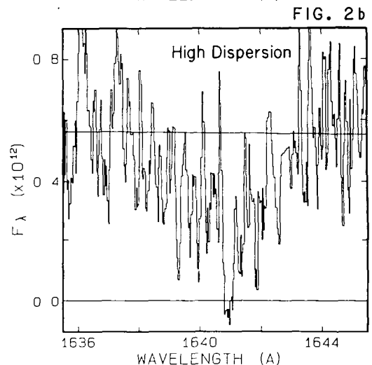
Fig. 2 The He II \lambda 1640 feature in PG1210+533. a) At low dispersion the pressure broadened component has an equivalent width of 3Å. b) At high dispersion a narrow saturated core is present, which is similar to non-LTE features seen in hot DO white dwarfs. This narrow feature has an equivalent width of 380 mÅ and a radial velocity of -5.8 \text{ km s}^{-1} . The sloping line in both plots is the same model atmosphere continuum.
