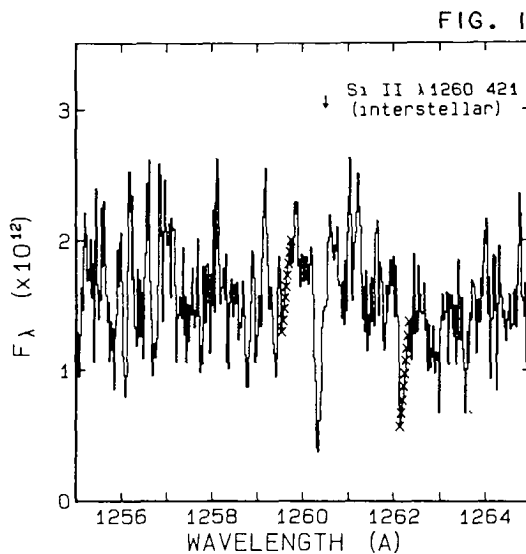
Fig. 1 An interstellar feature due to Si II \lambda 1260.421 . This is the only narrow metallic feature found in the high dispersion spectrum of PG1210+533. It has an equivalent width of 145 mÅ and a radial velocity of -16.6 \text{ km s}^{-1} .
