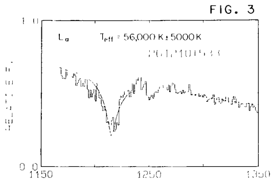
Fig. 3 The Ly \alpha profile of PG1210+533 obtained from the IUE small aperture image. The smooth curve is a model atmosphere fit yielding T_{\text{eff}} = 56,000 \text{ K} \pm 5000 \text{ K} .
