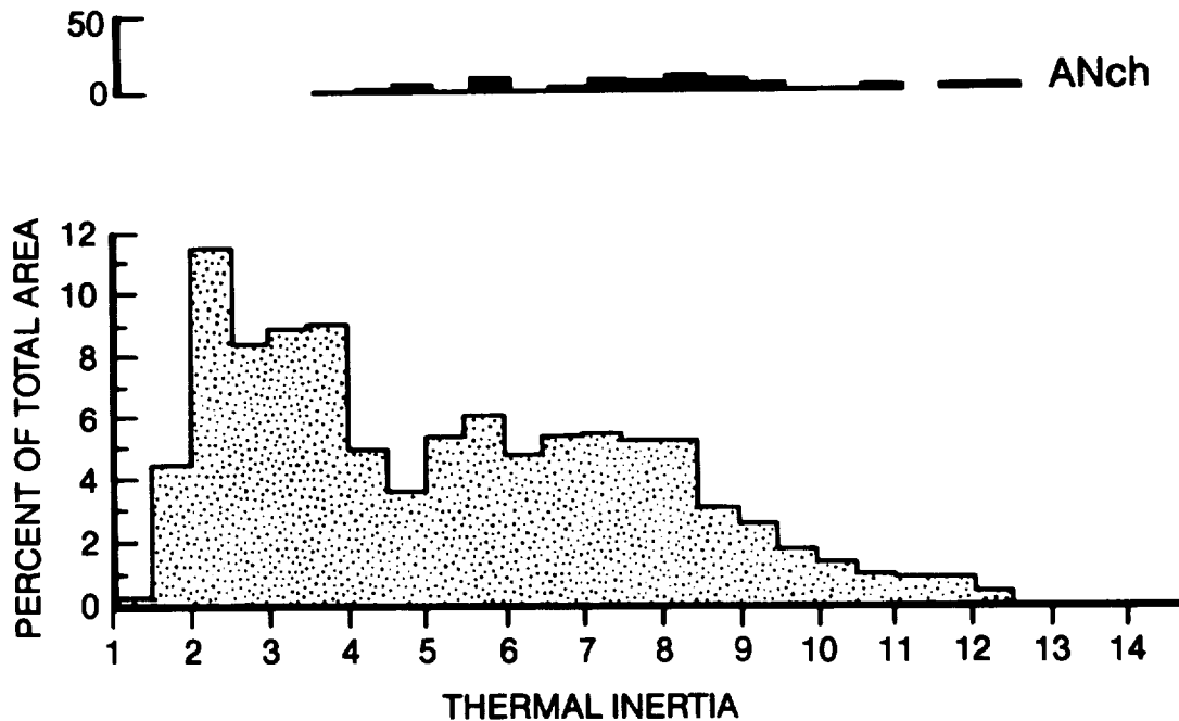
Fig. 3. Thermal inertias for channel material (top, solid) and all of the 1.7 \times 10^6 km 2 measured within the Elysium and Aeolis quadrangles with high resolution thermal data (bottom, stipled). Vertical axis on channel distribution is the number of 1/4^\circ by 1/4^\circ latitude-longitude bins having the thermal inertias indicated by the horizontal axis. Note the wide distribution of thermal inertias (in units of 10^{-3} cal cm -2 s -1/2 K -1 ) for the channel materials. The bimodal cumulative distribution results from predominantly low thermal inertias on the northern plains and predominantly high thermal inertias on the southern highlands. The unit name ANCh indicates that the age of the channels is from (A)mazonis to (N)oachian (4). Thermal data are from (2,6).
