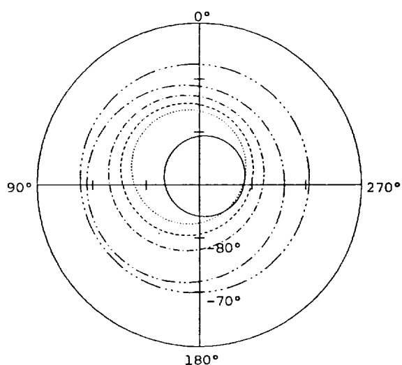
Fig. 2. South polar cap boundaries at L_s=245^\circ-254^\circ ----- 1909 ..... 1924 ——— 1926 ..... 1939 -.-.- 1941 ..... 1956
