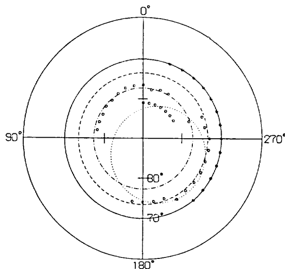
Fig. 3. North polar cap boundaries at L_s=65^\circ-74^\circ . ——— 1916 ..... 1948 ----- 1950 -.-.- 1965
