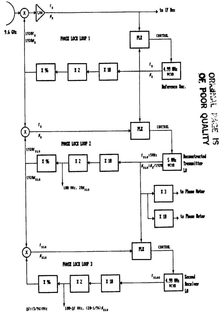
Figure 4. Block diagram of 9.6 GHz receiver and reconstruction of transmitter LO.
