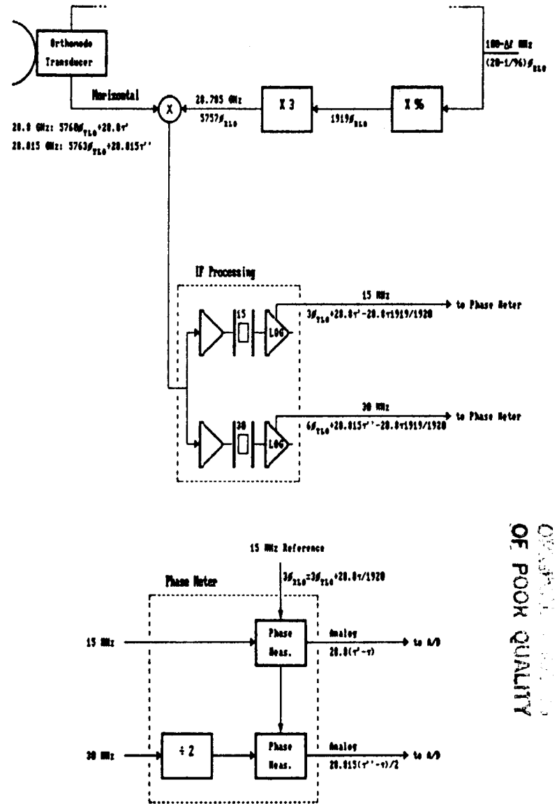
Figure 6. Example of phase analysis of 28.8 GHz receiver.
