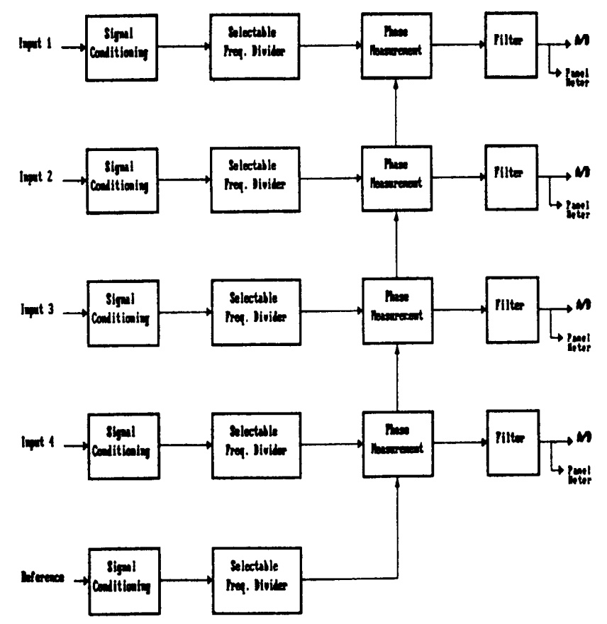
Figure 8. Block diagram of phase meters.
