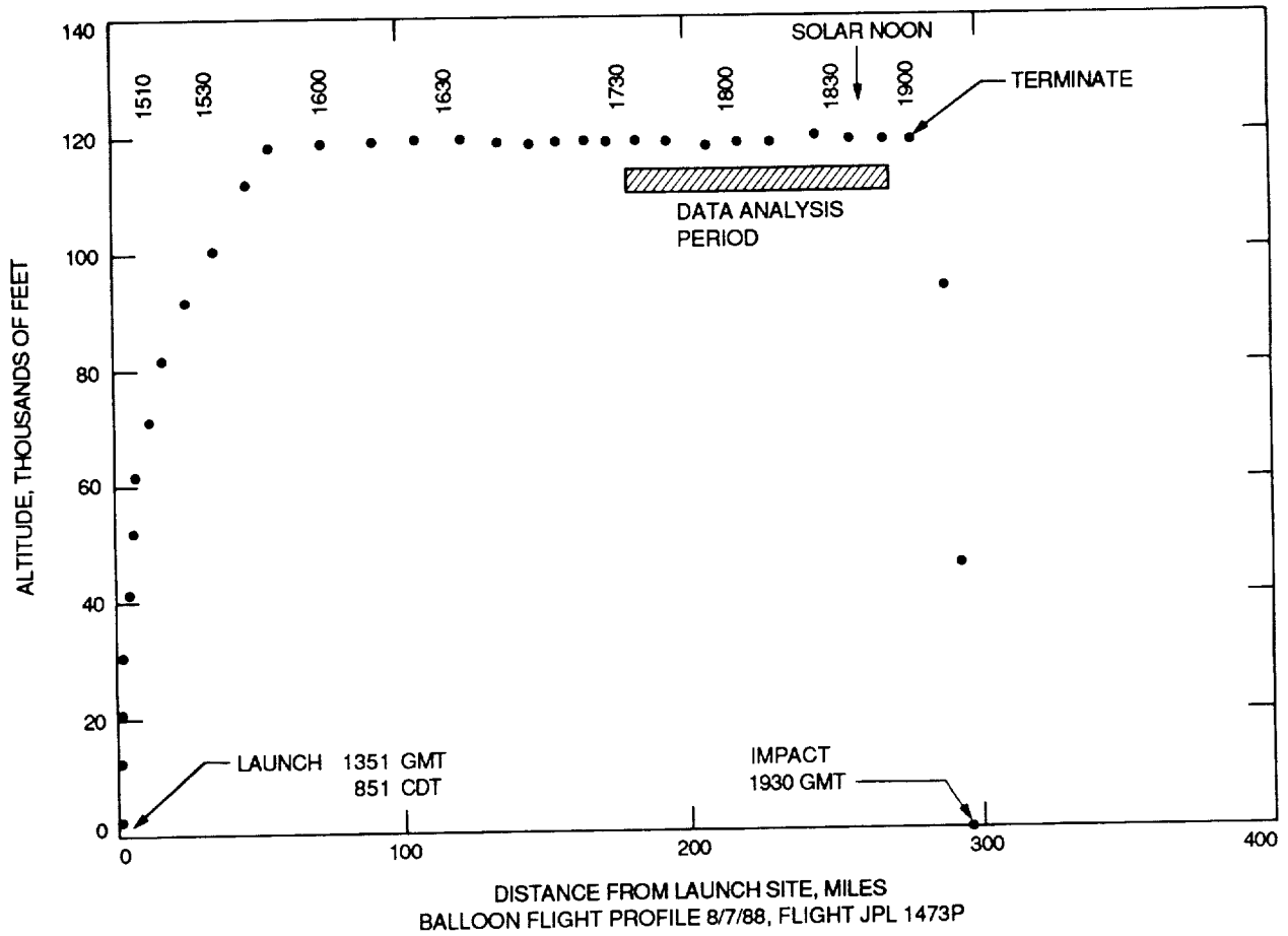
Figure 7. 1988 Balloon Flight Profile
