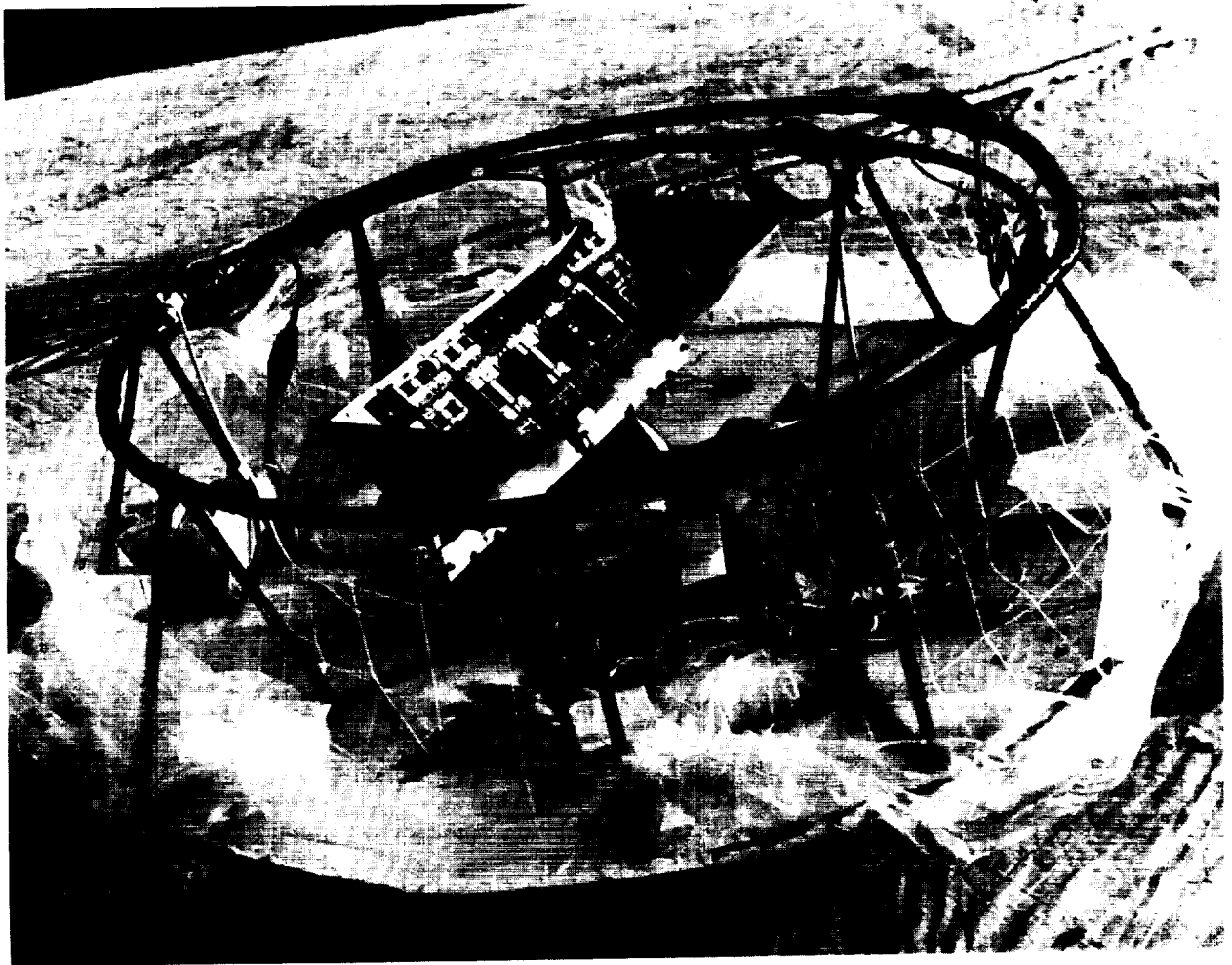
Figure 3. Aluminum Hoop Assembly with Tracker Mounted
