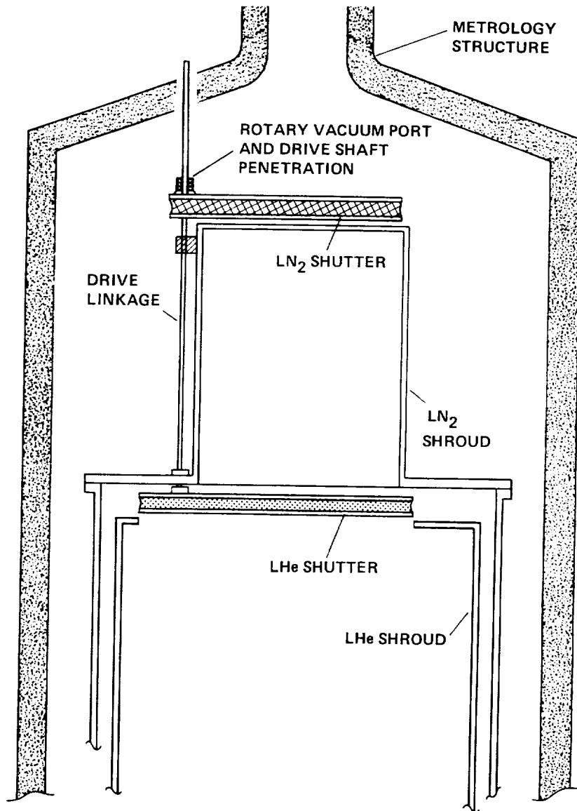
Figure 7.- Shutter concept.
