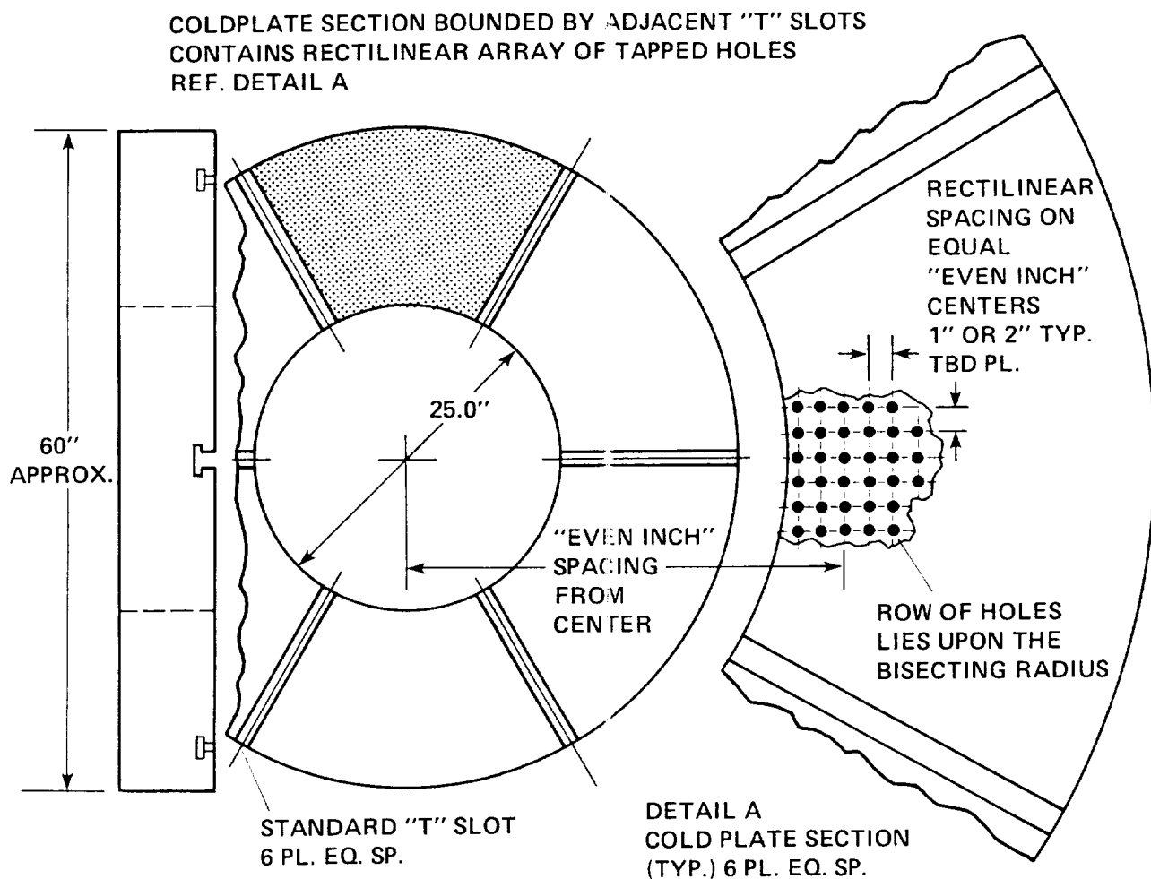
Figure 3.— Cold plate.
