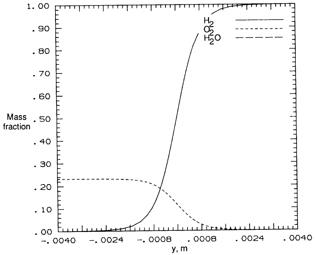
Figure 60. Mass fraction versus y at x = 0 cm.
