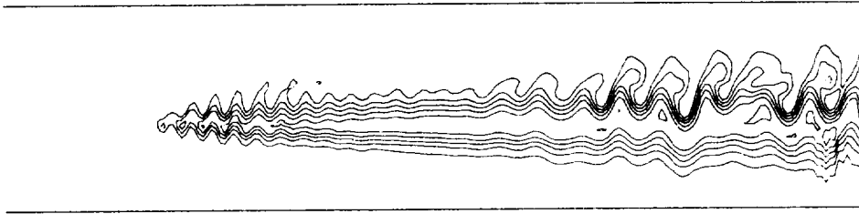
Figure 35. Water mass fraction contours in mixing layer.
