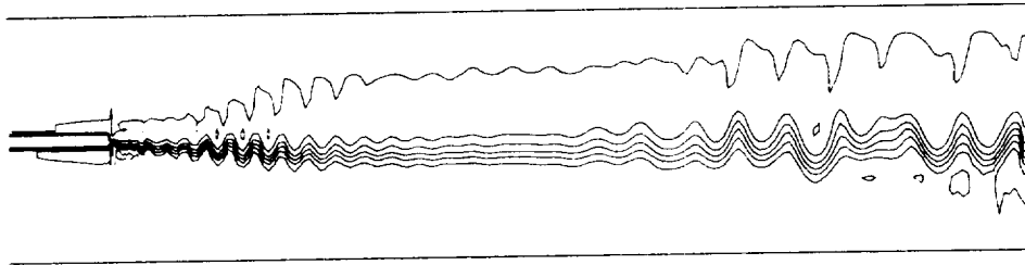
Figure 21. Temperature contours in mixing layer.
