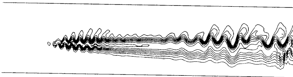
Figure 32. Atomic hydrogen (H) mass fraction contours in mixing layer.
