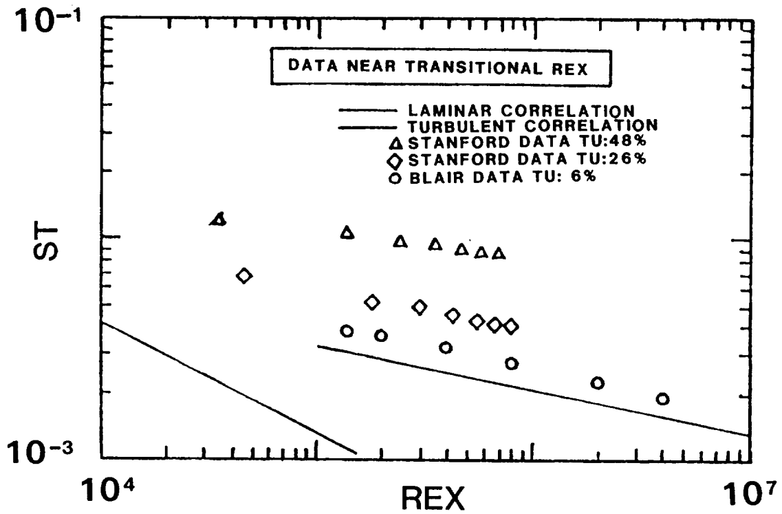
Fig. 2. High turbulence effects on heat transfer
