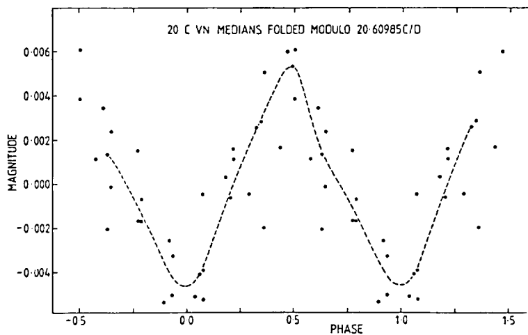
Figure 12 shows the mean light curve of 20 CVn using all 3 nights' data. A mean 2^{\text{h}} 55^{\text{m}} light curve has been removed but no other corrections have been applied. The r.m.s. scatter about the mean curve is \pm 0.0016 mags.
