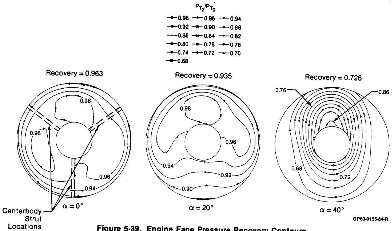
Figure 5-39. Engine Face Pressure Recovery Contours Baseline Configuration Axisymmetric Inlet M_0 = 0.9
