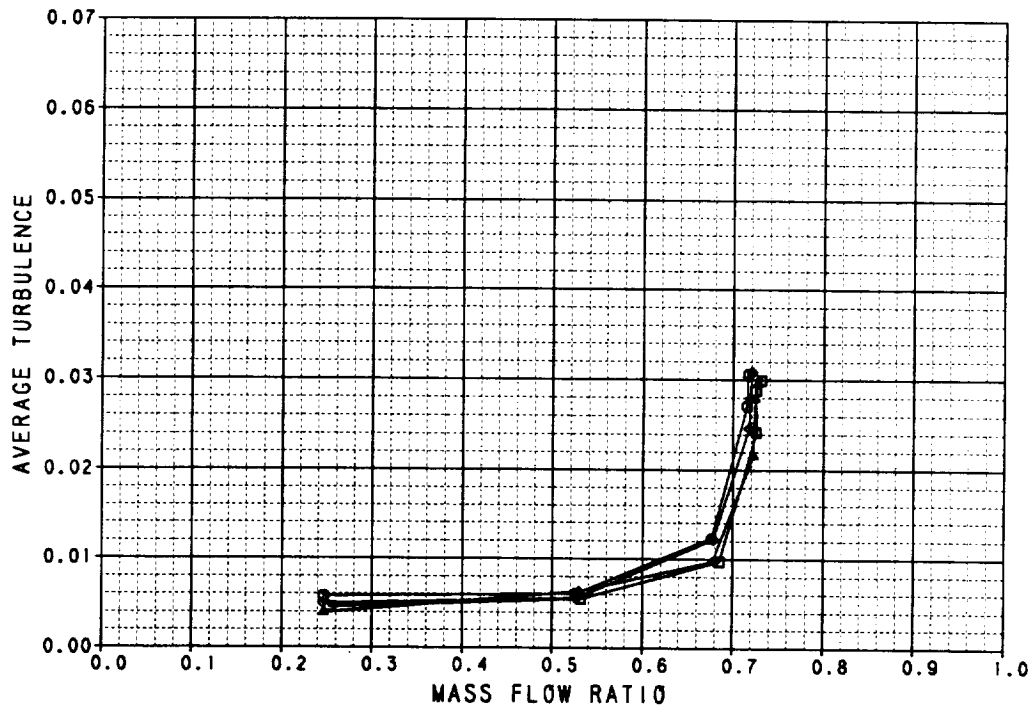
Figure B-7. Performance Data Axisymmetric Inlet With 20° Cowl Lip M_0 = 1.2
