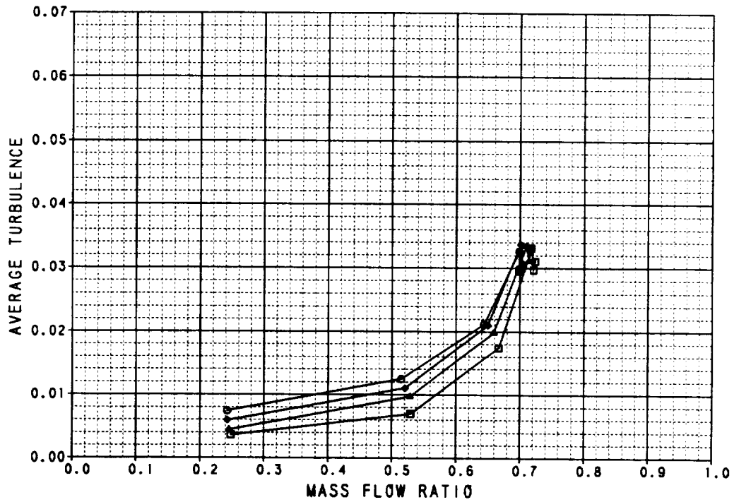
Figure B-11. Performance Data Axisymmetric Inlet With 40° Cowl Lip M_0 = 1.2
