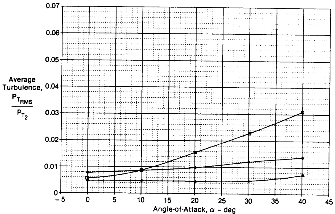
Figure 5-18. Effect of Rotating Cowl Lip on 2-D Inlet Recovery and Average Turbulence M_0 = 0.6
