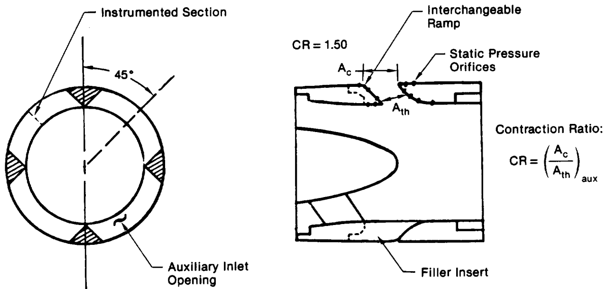
Figure 3-17. Auxiliary Inlet Section Instrumentation
