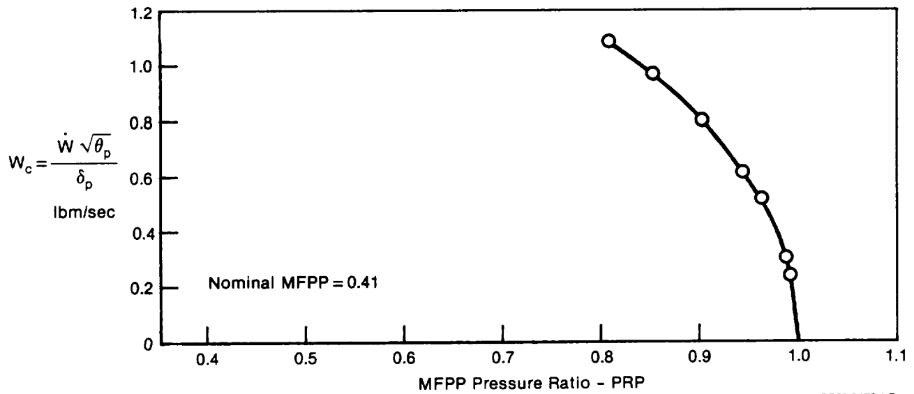
Figure A-3. NASA-Lewis HIMAT Mass Flow Plug Calibration Curves
