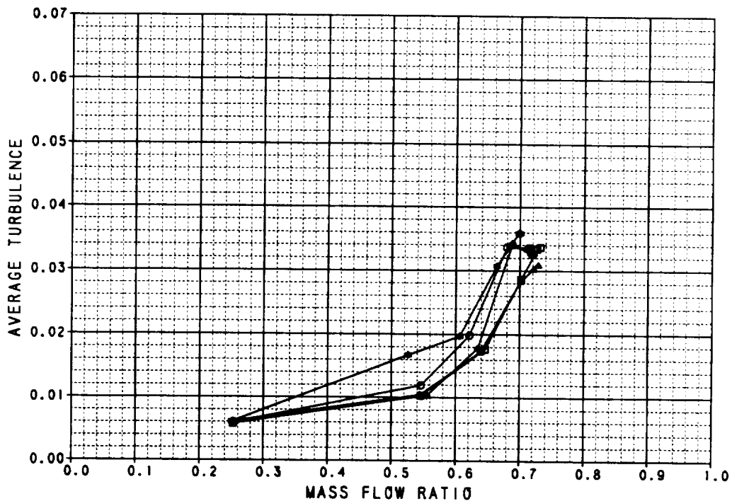
Figure B-31. Performance Data Axisymmetric Inlet Upper Auxiliary Inlets Open 100% M_0 = 1.4
