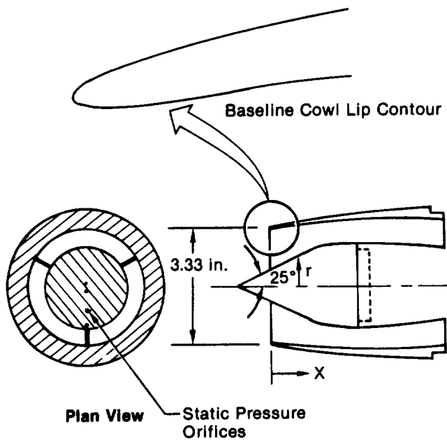
Figure 3-14. Main Inlet Section Design
