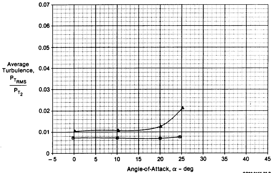
Figure 5-65. Comparison of 2-D and Axisymmetric Inlets M_0 = 1.2
