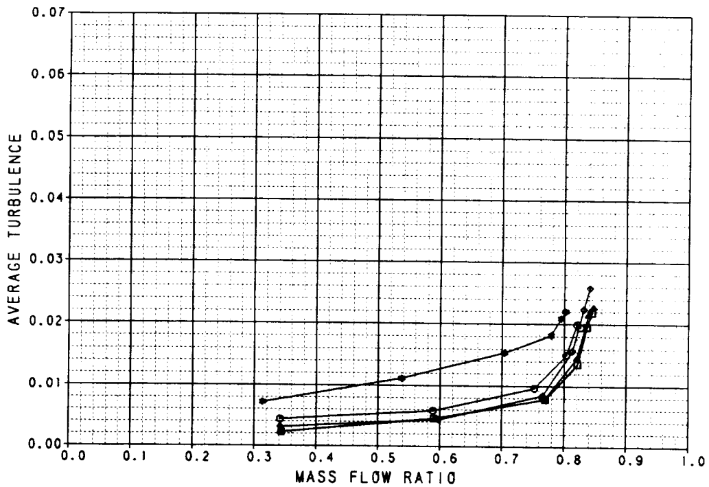
Figure B-5. Performance Data Axisymmetric Inlet With 20° Cowl Lip M_0 = 0.6
