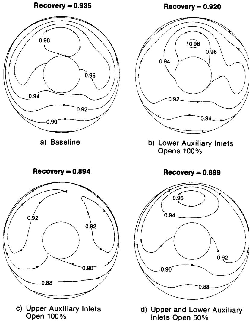
Figure 5-57. Comparison of Axisymmetric Inlet Engine Face Pressure Recovery Contours Auxiliary Inlet Configurations M_0 = 0.9 \alpha = 20^\circ
