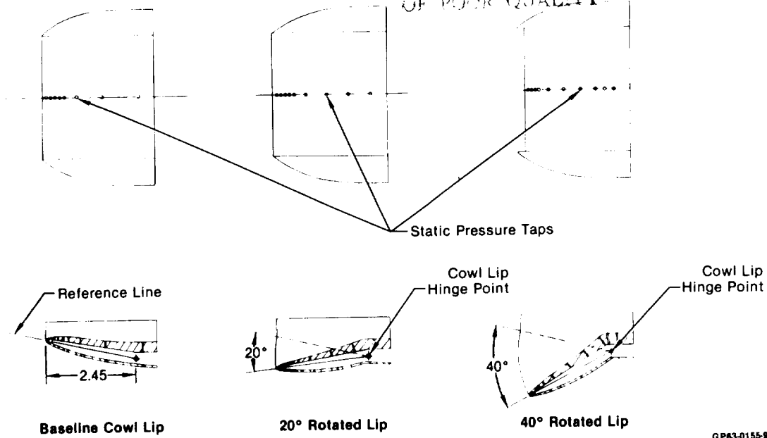
Figure 3-8. 2-D Inlet Rotated Cowl Lip Configurations
