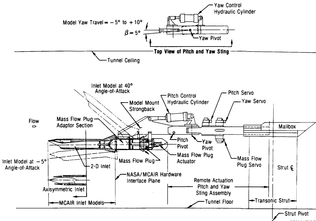
Figure 2-2. MCAIR Highly Maneuverable Inlet Model Installation NASA-Lewis Research Center 8 x 6 Ft Wind Tunnel
