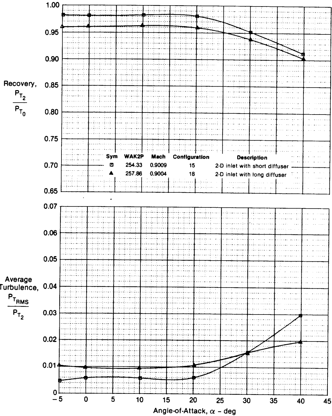
Figure 5-13. Effect of Diffuser Length on 2-D Inlet Recovery and Average Turbulence M_0 = 0.9
