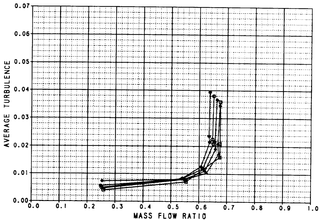
Figure B-15. Performance Data Axisymmetric Inlet With Retracted Sideplates M_0 = 1.4
