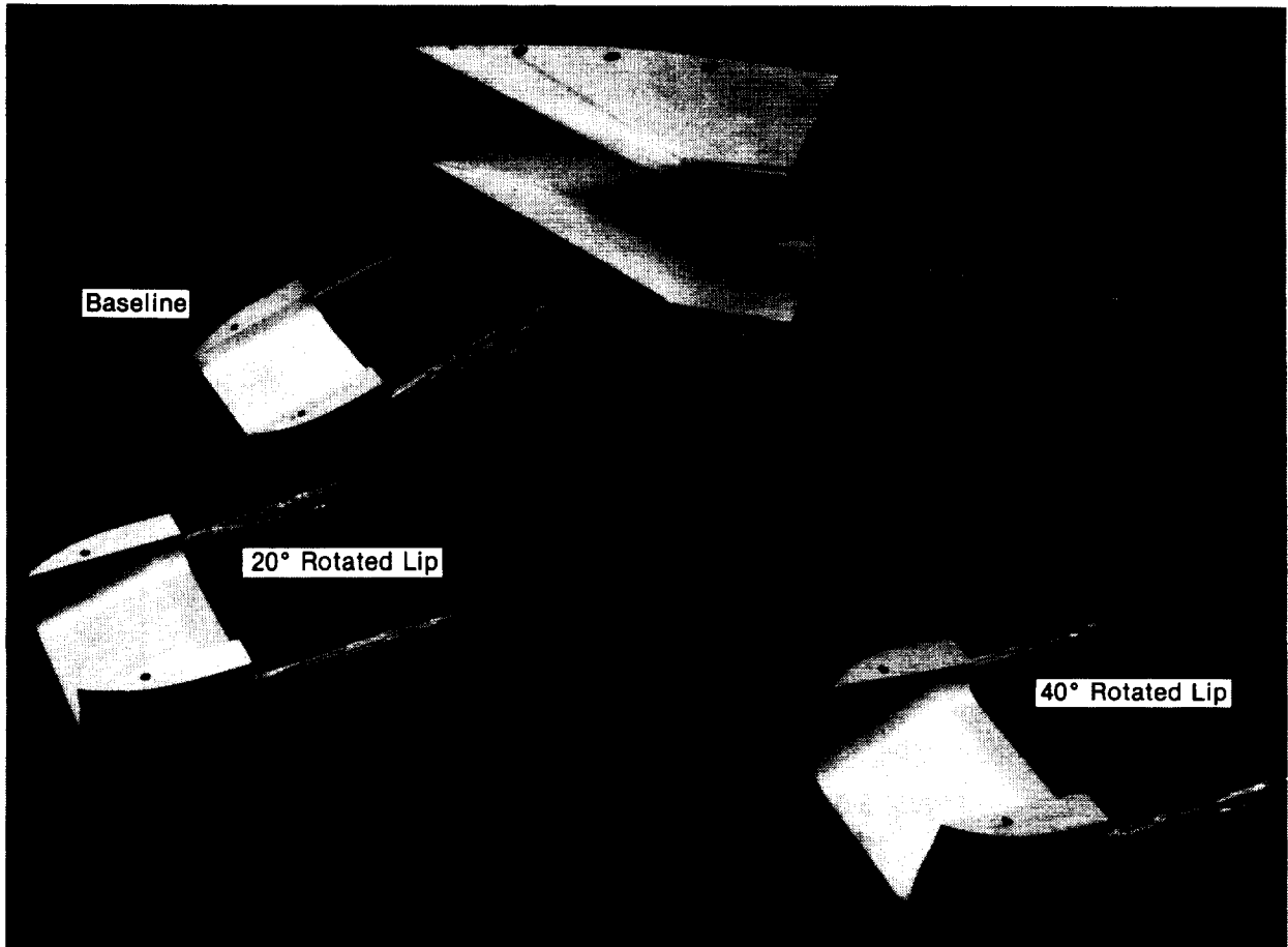
Figure 3-7. 2-D Inlet Lower Cowl Lip Variations
