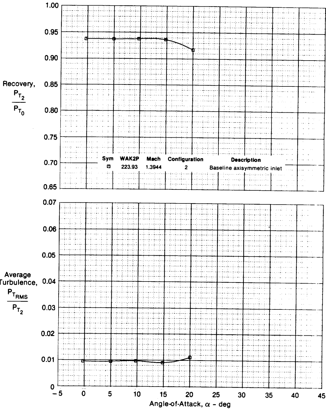
Figure 5-40. Baseline Axisymmetric Inlet Recovery and Average Turbulence vs Angle-of-Attack M_0 = 1.4
