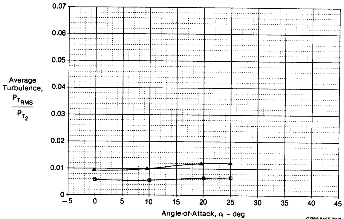
Figure 5-68. Comparison of 2-D and Axisymmetric Inlets 20° Rotated Cowl Lip Configurations M_0 = 1.2
