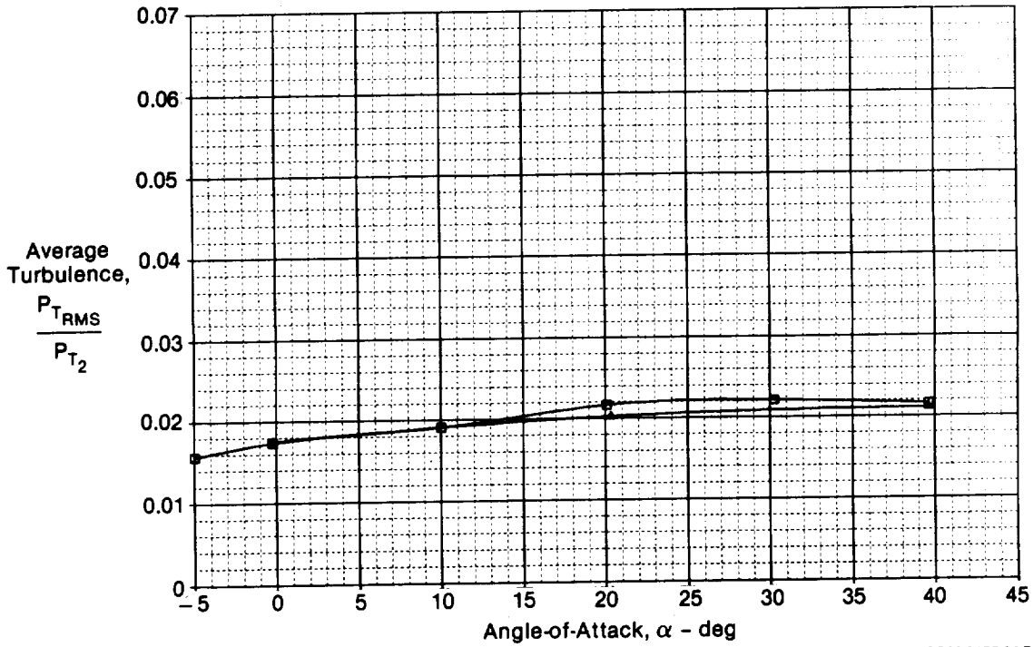
Figure 5-47. Effect of Blunt and Sharp Highlights on 40° Rotated Lip Recovery and Average Turbulence M_0 = 0.9
