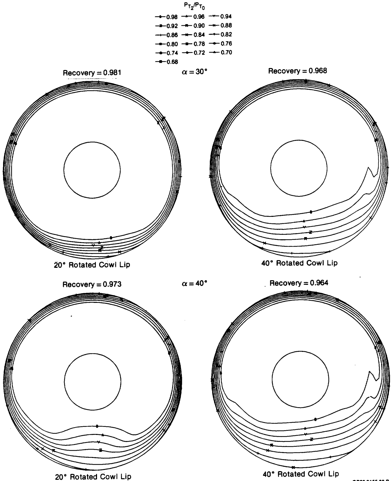
Figure 5-21. Comparison of Engine Face Pressure Recovery Contours 20° and 40° Rotated Cowl Lips 2-D Inlet M_0 = 0.6 \quad \alpha = 30^\circ, 40^\circ
