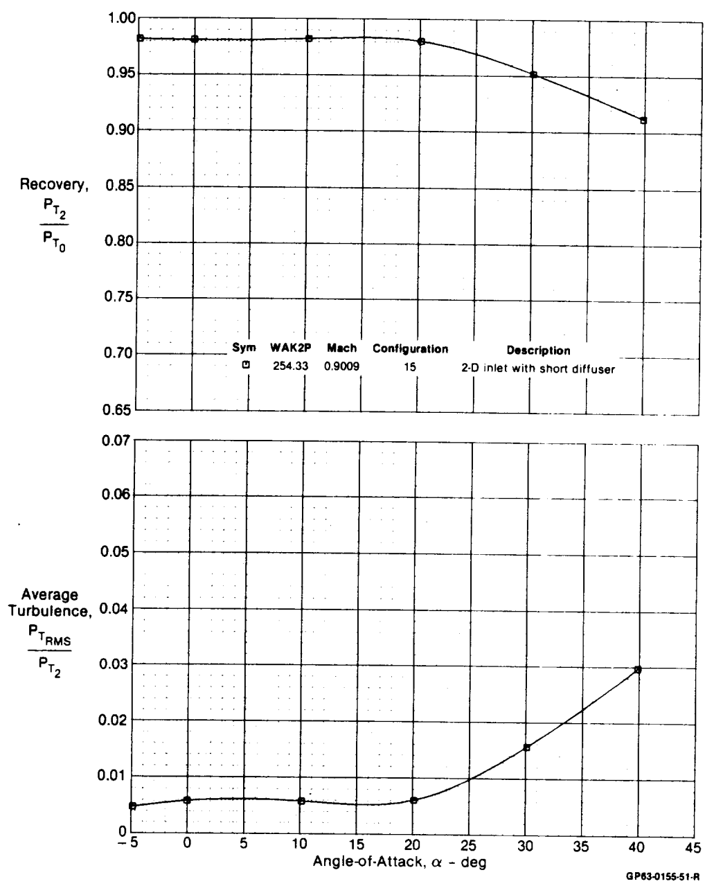
Figure 5-4. Baseline 2-D Inlet Recovery and Average Turbulence vs Angle-of-Attack M_0 = 0.9
