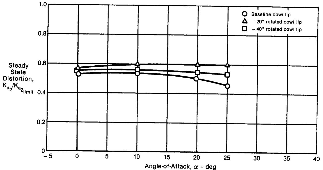
Figure 5-26. Effect of Rotating Cowl Lip on 2-D Inlet Distortion Mach 1.2
