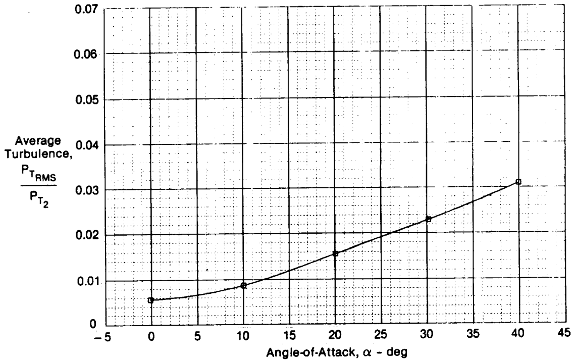
Figure 5-1. Baseline 2-D Inlet Recovery and Average Turbulence vs Angle-of-Attack M_0 = 0.6
