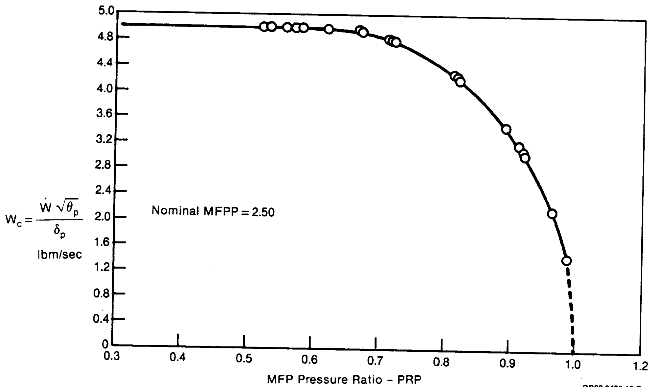
Figure A-3. (Concluded) NASA-Lewis HIMAT Mass Flow Plug Calibration Curves
