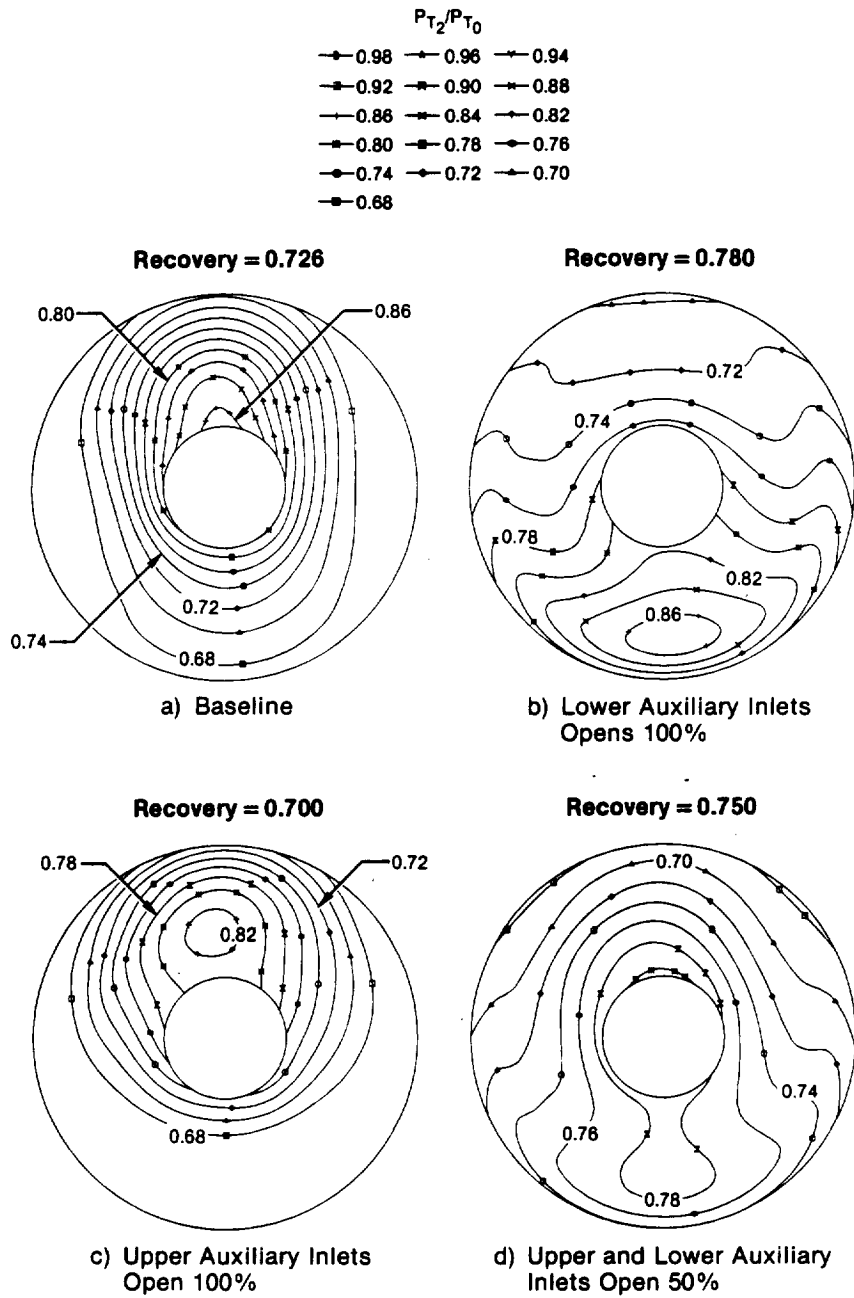
Figure 5-58. Comparison of Axisymmetric Inlet Engine Face Pressure Recovery Contours Auxiliary Inlet Configurations M_0 = 0.9 \alpha = 40^\circ
