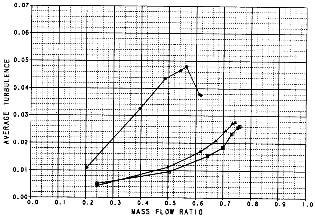
Figure B-23. Performance Data Axisymmetric Inlet Upper and Lower Auxiliary Inlets Open 50% M_0 = 0.9
