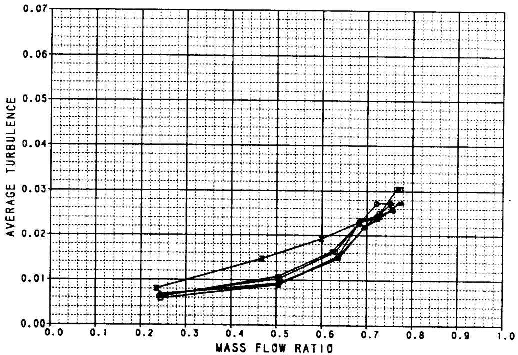
Figure B-37. Performance Data Axisymmetric Inlet 20° Cowl Lip Lower Auxiliary Inlets Open 100% M_0 = 0.9
