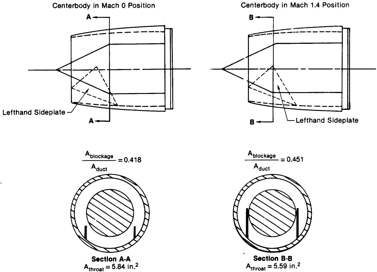
Figure 5-52. Blockage Ratios for the Two Axisymmetric Inlet Centerbody Positions With Retracted Sideplates
