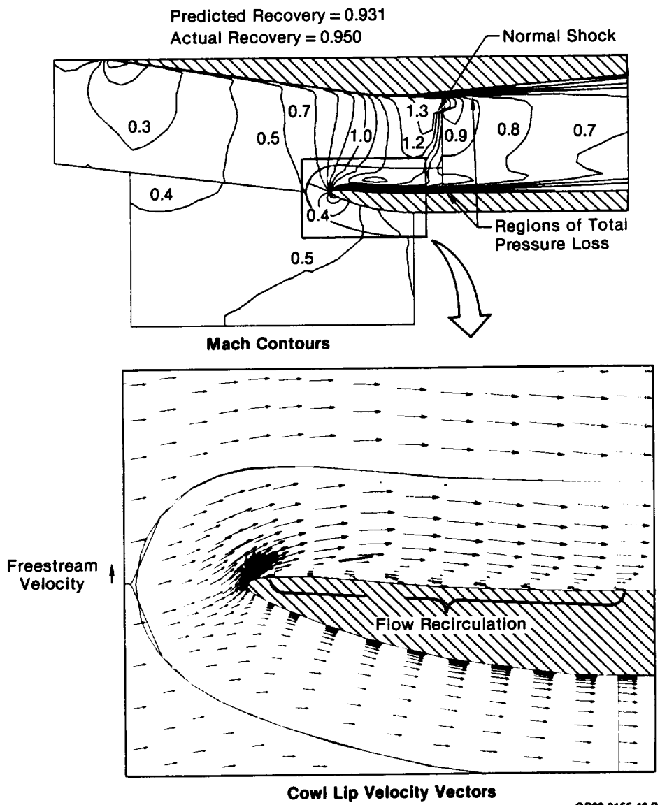
Figure 5-29. Baseline Configuration, Computed Flowfield M_0 = 0.6 \alpha = 20^\circ
