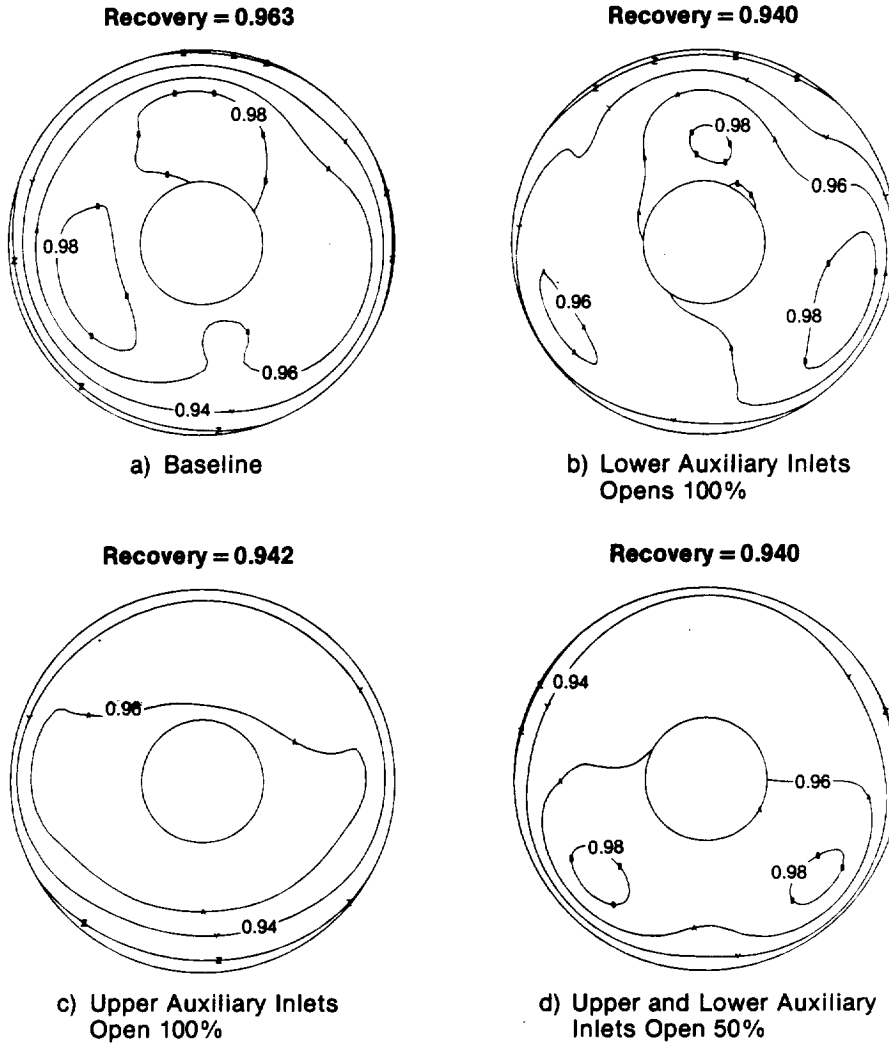
Figure 5-56. Comparison of Axisymmetric Inlet Engine Face Pressure Recovery Contours Auxiliary Inlet Configurations M_0 = 0.9 \alpha = 0^\circ
