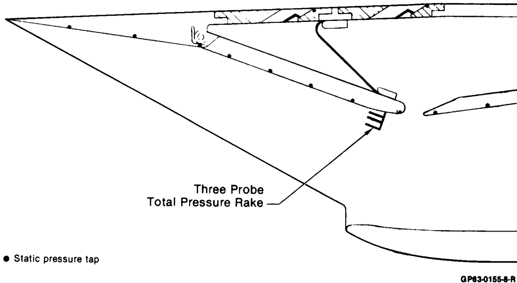
Figure 3-6. 2-D Inlet Model Instrumentation Long Diffuser Configuration
