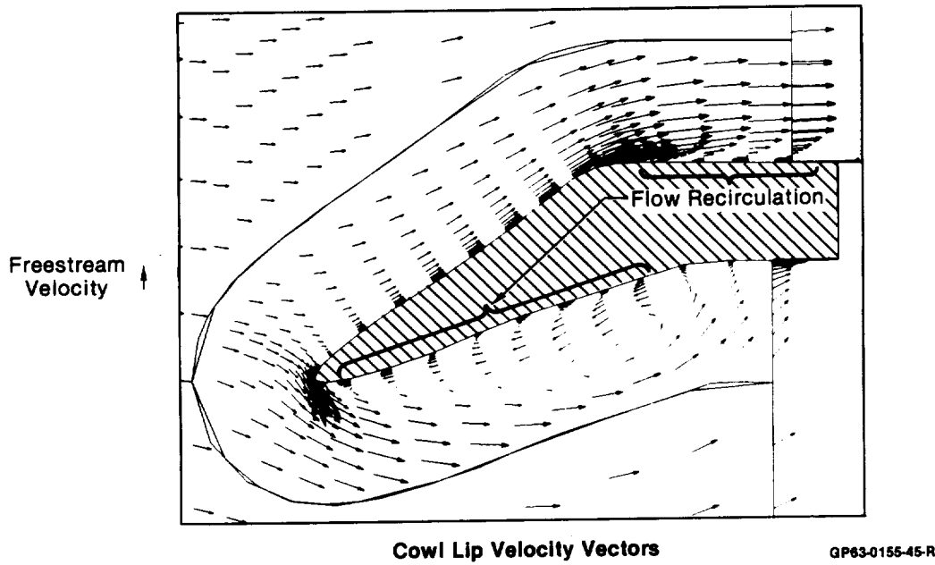
Figure 5-32. 40° Rotated Lip Configuration, Computed Flowfield M_0 = 0.6 \alpha = 0^\circ
