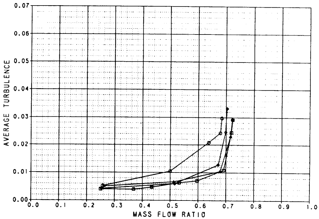
Figure B-3. Performance Data Baseline Axisymmetric Inlet M_0 = 1.2
