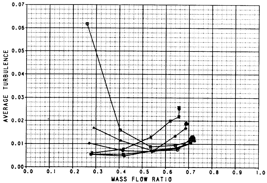
Figure B-51. Performance Data 2-D Inlet With Long Diffuser M_0 = 0.9
