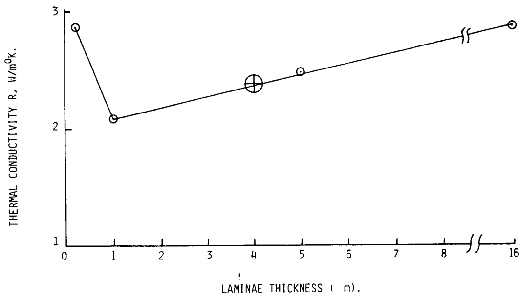
Thermal Conductivity (direction \perp to laminae plane) vs. laminae thickness for MCrAlY - \alpha -Al 2 O 3 microlaminates.
