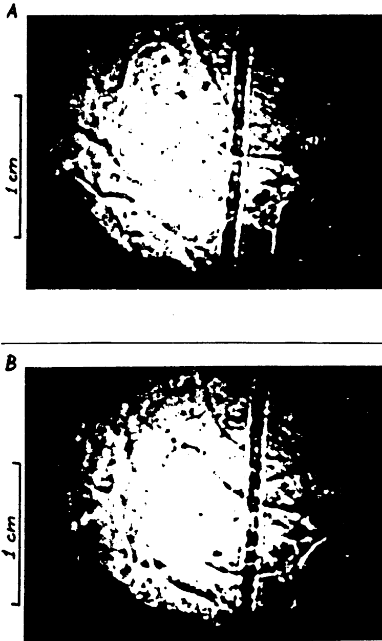
Figure 5. Shadowgraph of solidifying off-eutectic melt. Visible rising plumes caused by double diffusive phenomena. Chill placed beyond field of view to the right. Time of photograph reported in minutes from beginning of experiment: (a) 20 and (b) 20.17.
