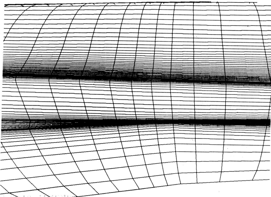
Figure 6.— Enlarged view near the beginning of notch, (a) singular case, (b) non-singular case.
