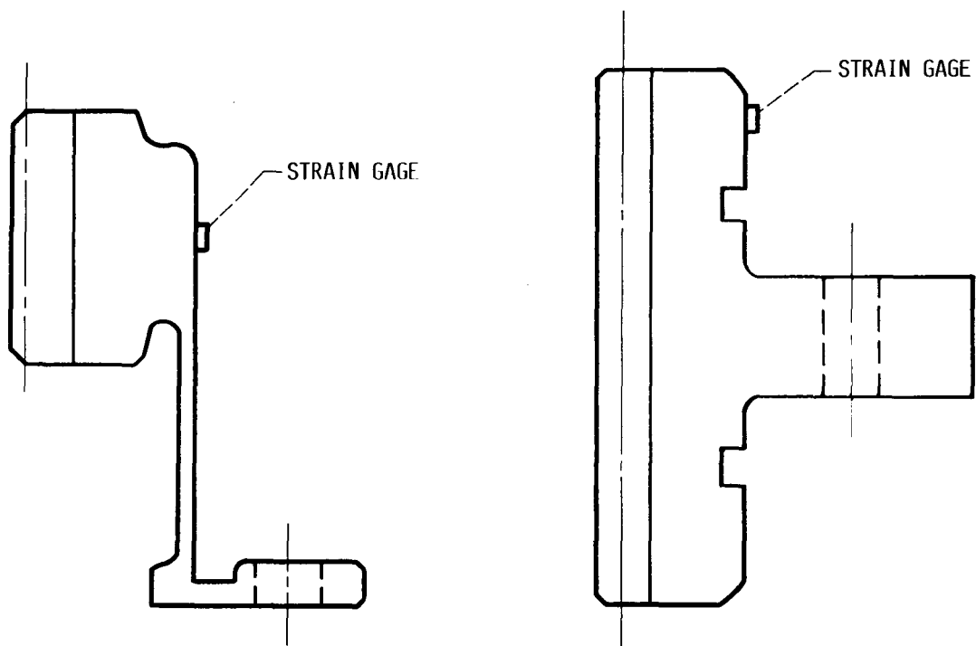
(a) FLEXIBLE RING GEAR, ADVANCED TECHNOLOGY TRANSMISSION.
