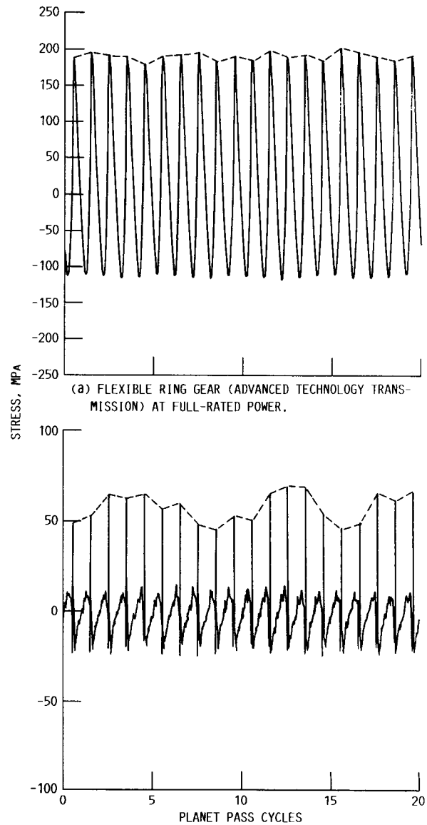
(a) FLEXIBLE RING GEAR (ADVANCED TECHNOLOGY TRANSMISSION) AT FULL-RATED POWER. (b) RIGID RING GEAR (UH-60A TRANSMISSION) AT FULL-RATED POWER.
