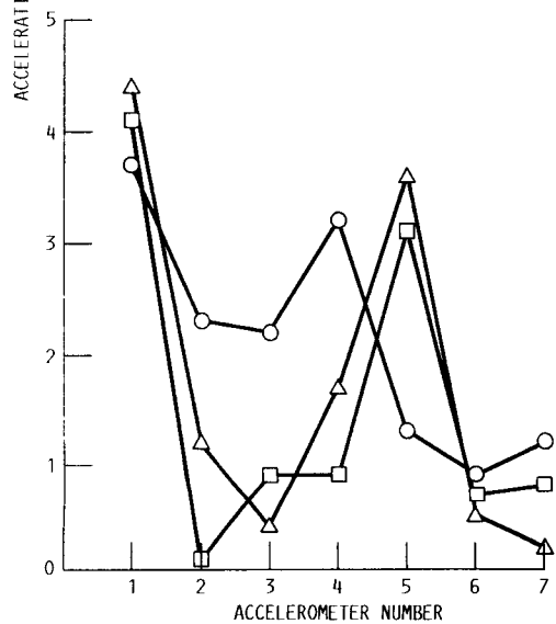
(a) PLANETARY MESH VIBRATION LEVELS. (b) SPIRAL-BEVEL MESH VIBRATION LEVELS. FIGURE 8. - PLANETARY AND SPIRAL-BEVEL MESH VIBRATION LEVELS OF OH-58A, OH-58C, AND ADVANCED TECHNOLOGY TRANSMISSION. OH-58A AND OH-58C AT 224 kW AND 6060 RPM, ATT AT 233 kW AND 6180 RPM.
