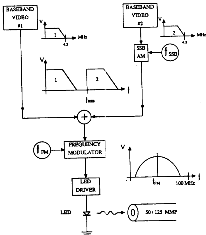
Figure 4-2. Scheme 2: AM/FDM
