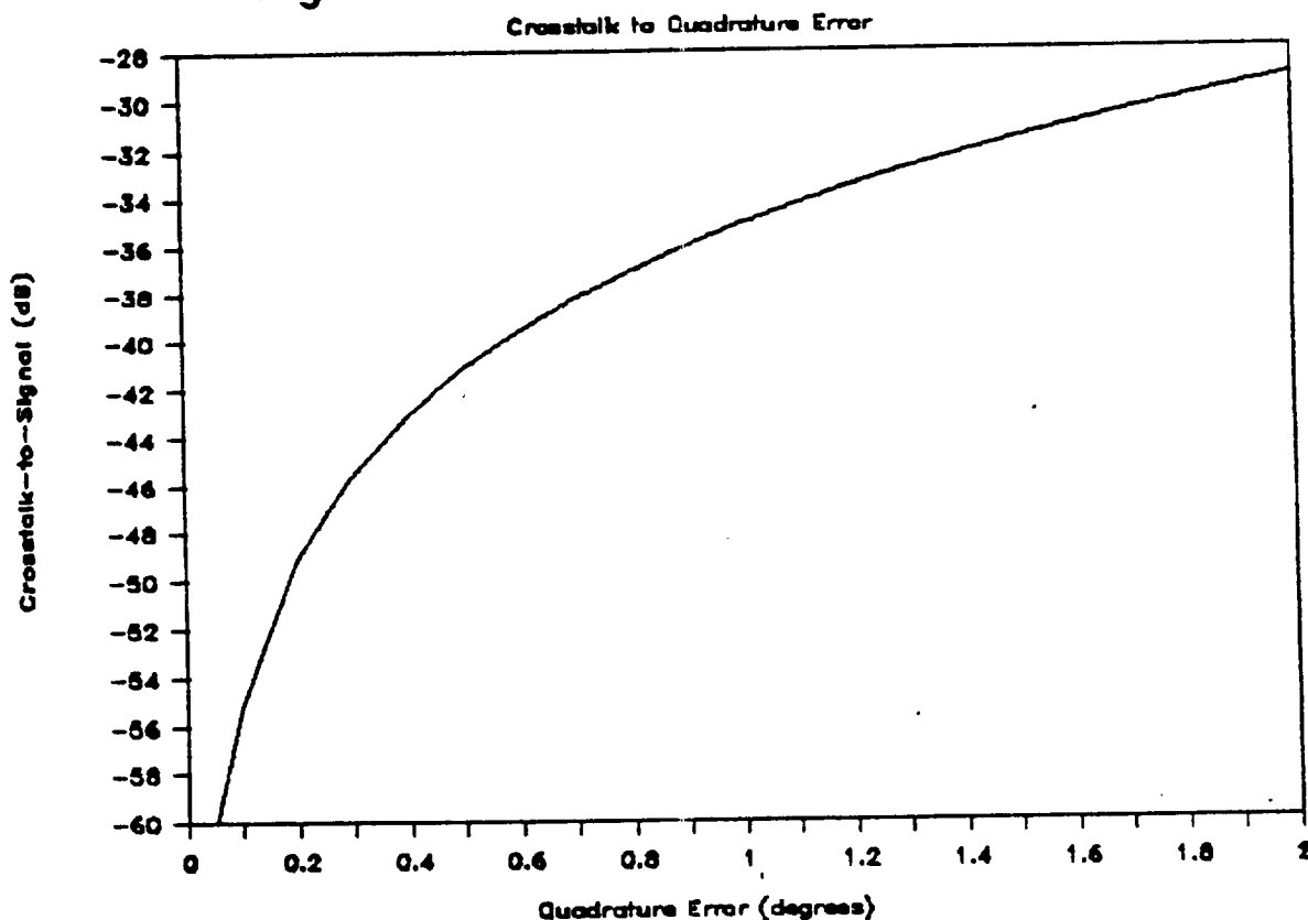
Figure 5-10 QAM Phase Sensitivity
