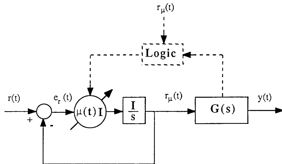
Figure 3.2: The basic system for calculating \mu(t) .
