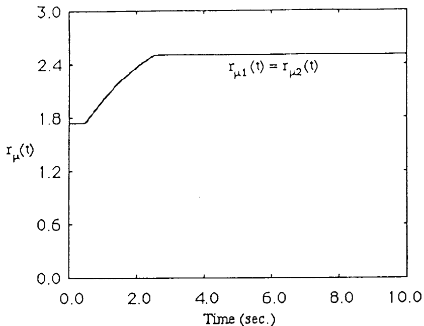
Figure 4.17: r_{\mu}(t) in the F16 system with saturation and the RG, ( r = [2.5 \quad 2.5]^T ).
