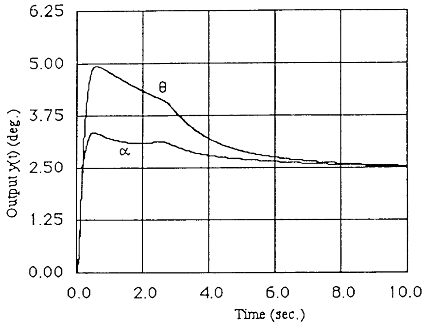
Figure 4.15: Output response for the F16 system with saturation and the RG, ( r = [2.5 \ 2.5]^T ).
