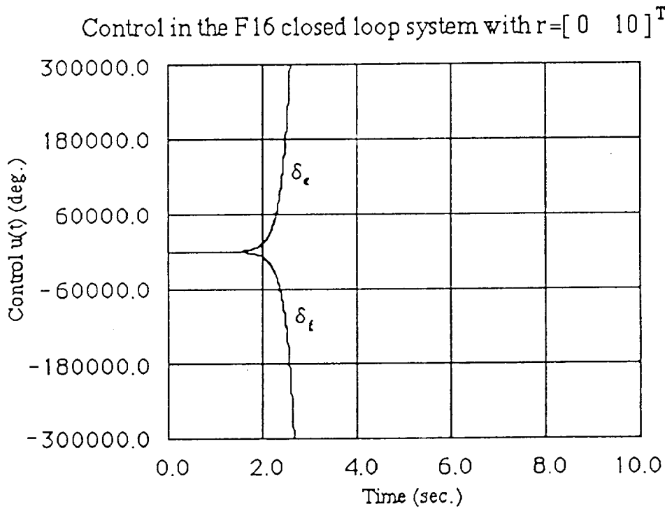
Figure 4.7: Controls in the F16 system with saturation, ( r = [0 \ 10]^T ).
