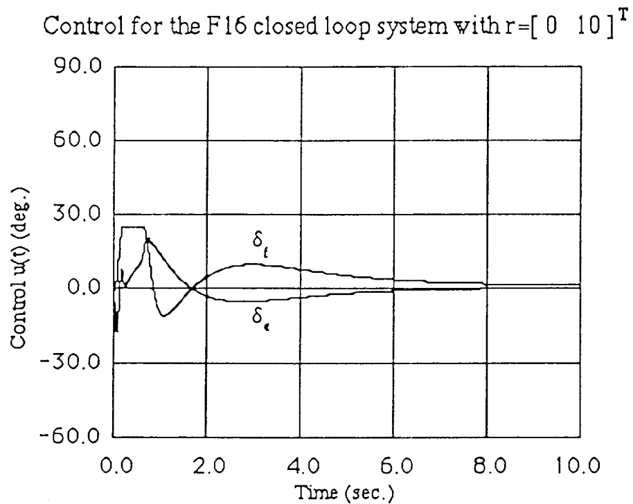
Figure 4.9: Controls in the F16 system with saturation and the RG, ( r = [0 \ 10]^T ).
