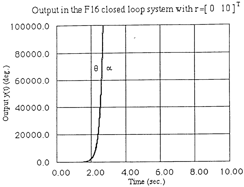
Figure 4.6: Output response of the F16 system with saturation, ( r = [0 \ 10]^T ).
