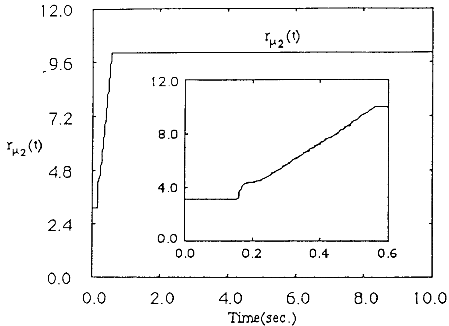
Figure 4.10: r_{\mu_2}(t) , the commanded pitch, in the F16 system with saturation and the RG, ( \mathbf{r} = [0 \quad 10]^T ). Insert: Blowup with 0 \leq t \leq .6 .
