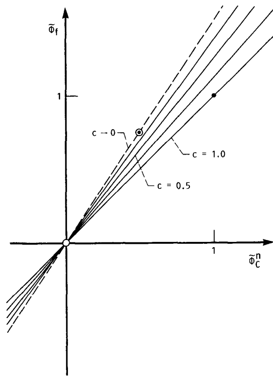
FIGURE 16. - NVD FOR SECOND-ORDER UPWINDING; \tilde{\phi}_f AS A FUNCTION OF \tilde{\phi}_C^n FOR c=0 , c=0.25 , 0.5 , 0.75 , AND 1 .
