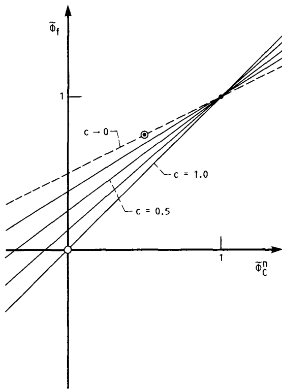
FIGURE 15. - NORMALIZED VARIABLE DIAGRAM (NVD) FOR THE LAX-WENDROFF METHOD; \tilde{\phi}_f AS A FUNCTION OF \tilde{\phi}_C^n FOR c=0 , c=0.25 , 0.5 , 0.75 , AND 1 .
