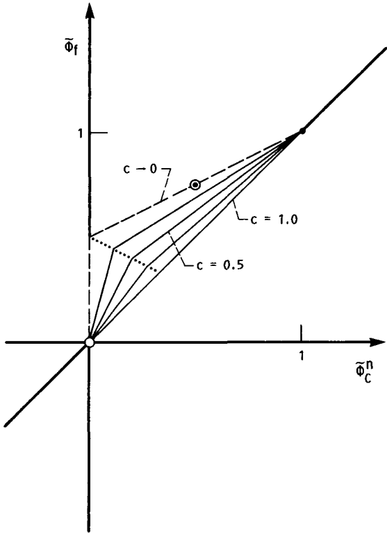
FIGURE 34. - NVD SHOWING \tilde{\phi}_f AS A FUNCTION OF \tilde{\phi}_c^n AND c FOR THE ULTIMATE LAX-WENDROFF METHOD.
