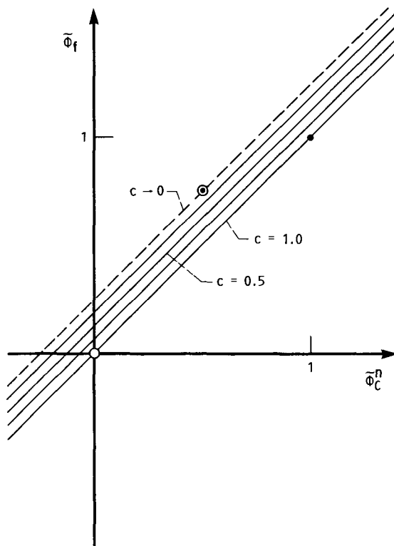
FIGURE 17. - NVD FOR FROMM'S METHOD; \tilde{\phi}_f AS A FUNCTION OF \tilde{\phi}_C^n FOR c=0 , c=0.25 , 0.5 , 0.75 , AND 1 .
