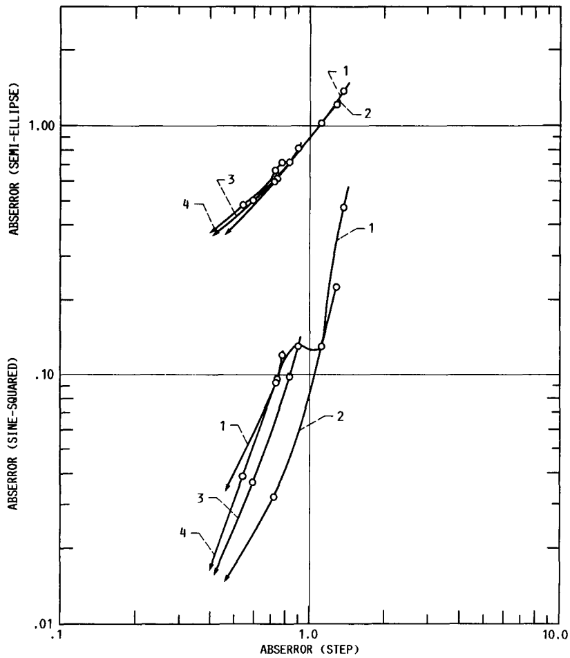
FIGURE 47. - ABSERROR FOR THE SEMI-ELLIPSE PROFILE (UPPER CURVES) AND SINE-SQUARED PROFILE (LOWER CURVES) PLOTTED ON A LOG-LOG SCALE AGAINST ABSERROR FOR THE STEP, WITH COURANT NUMBER AS A PARAMETER RANGING FROM 0.01 TO 0.098, WITH VALUES SHOWN AT 0.1, 0.5, AND 0.9. CURVES SHOW: (1) ULTIMATE FROMM, (2) ULTIMATE QUICKEST, (3) ULTIMATE FIFTH-ORDER UPWINDING, AND (4) ULTIMATE SEVENTH-ORDER UPWINDING. ARROWS SHOW DIRECTION OF INCREASING COURANT NUMBER.
