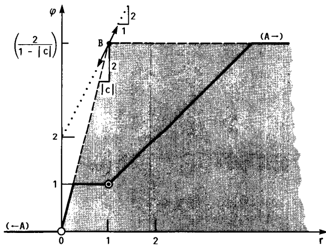
FIGURE A.2. - "EXTENDED SWEBY DIAGRAM" CORRESPONDING TO THE ULTIMATE STRATEGY OF FIGURE 33. FOR REFERENCE, THE SUPER-C SCHEME IS SHOWN BY THE HEAVY PIECEWISE LINEAR CHARACTERISTIC.
