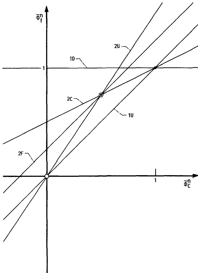
FIGURE 14. - NORMALIZED VARIABLE DIAGRAM SHOWING \bar{\phi}_f^n AS A FUNCTION OF \bar{\phi}_c^n FOR FIRST-ORDER UPWINDING (1U), LAX-WENDROFF (2C), SECOND-ORDER UPWINDING (2U), FROMM'S METHOD (2F), AND FIRST-ORDER DOWNWINDING (1D).
