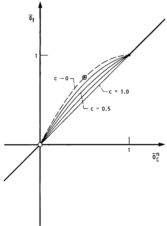
(b) \bar{\phi}_f AS A FUNCTION OF \bar{\phi}_c^n AND c .
