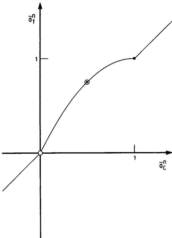
(a) \bar{\phi}_f^n AS A FUNCTION OF \bar{\phi}_c^n .
