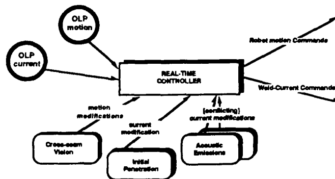
Figure 5: Pre-programmed motion and weld-process values are combined during weld execution with multiple sensor values.
