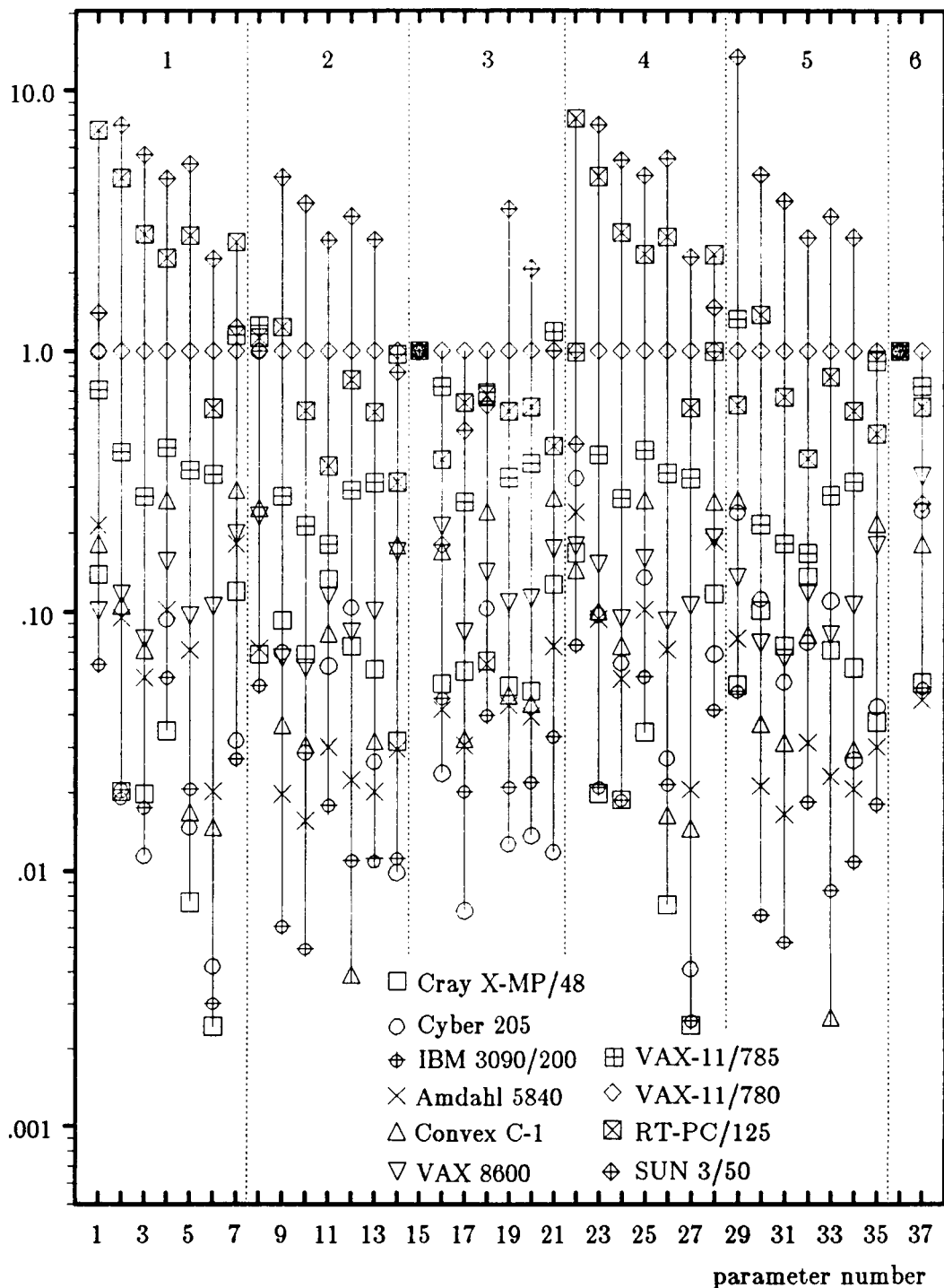
Figure 4.10: Characterization results for all machines normalized to the VAX-11/780 (I). Regions 1-6 represent different aspects of the characterization (see table 4.11).
