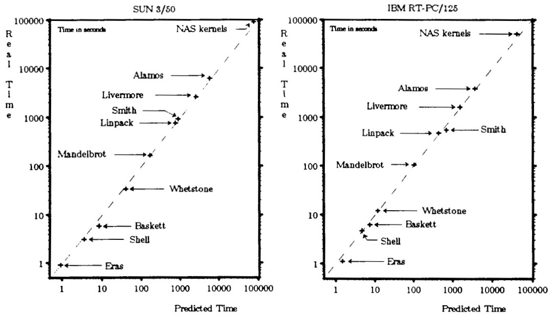
Figure 8.4: Predicted times versus real execution times (III). Results for the SUN 3/50, and the IBM RT-PC/125. Scales are logarithmic and values are reported in seconds.
