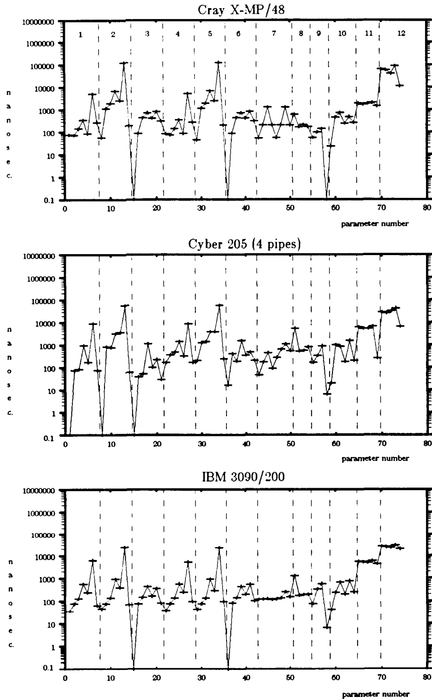
Figure 4.6: Characterization results (Cray, Cyber, and IBM 3090). The graphs show the value of each parameter in nanoseconds. The twelve regions represent different aspects of the characterization.
