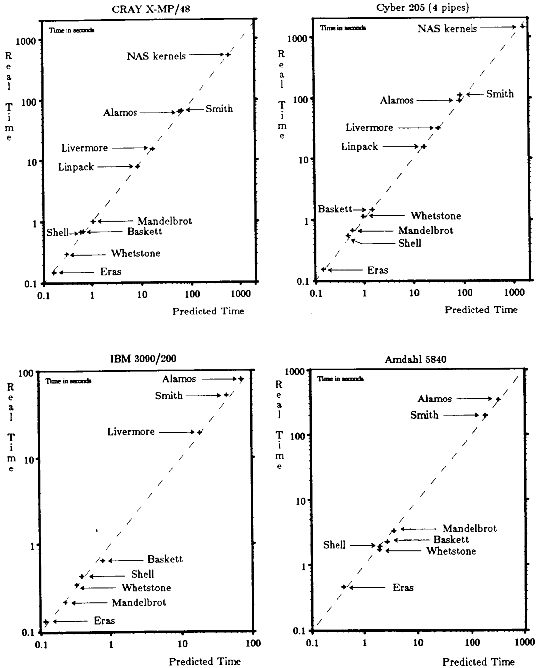
Figure 6.2: Predicted times versus real execution times (I). Results for the CRAY X-MP/48, the CYBER 205 (4 pipes), the IBM 3090/200, and the Amdahl 5840. Scales are logarithmic and values are reported in seconds.
