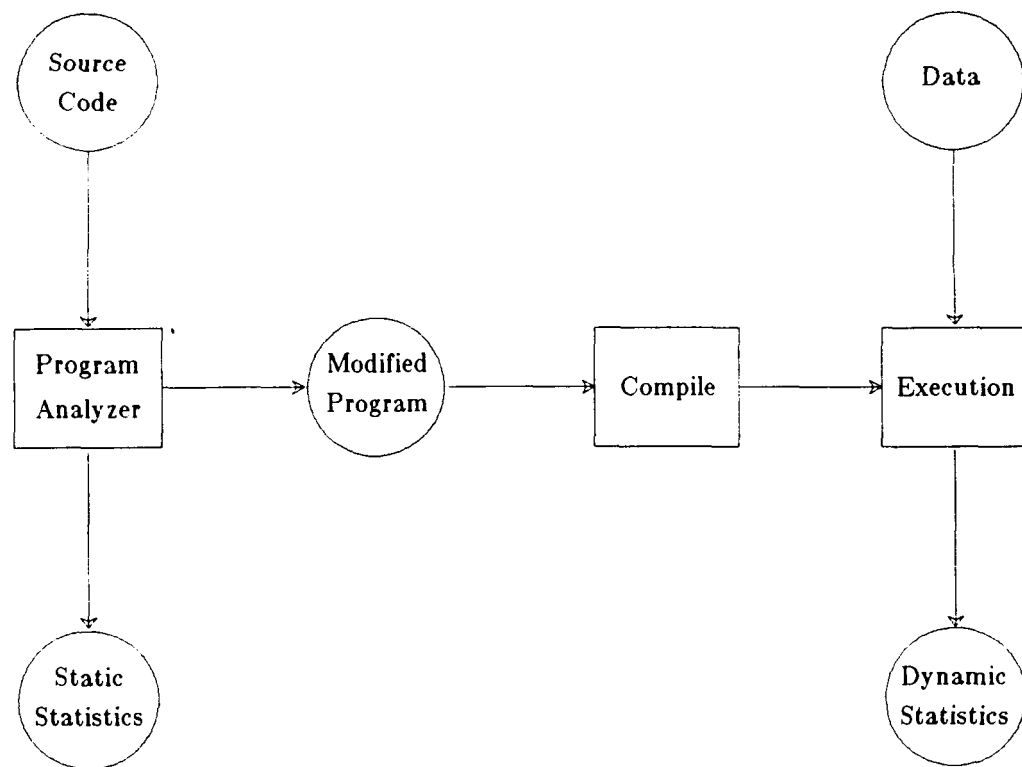
Figure 5.1: Static and dynamic analysis of programs.
