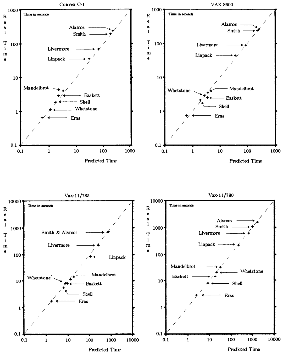
Figure 6.3: Predicted times versus real execution times (II). Results for the Convex C-1, the VAX 8600, the VAX-11/785, and the VAX-11/780. Scales are logarithmic and values are reported in seconds.
