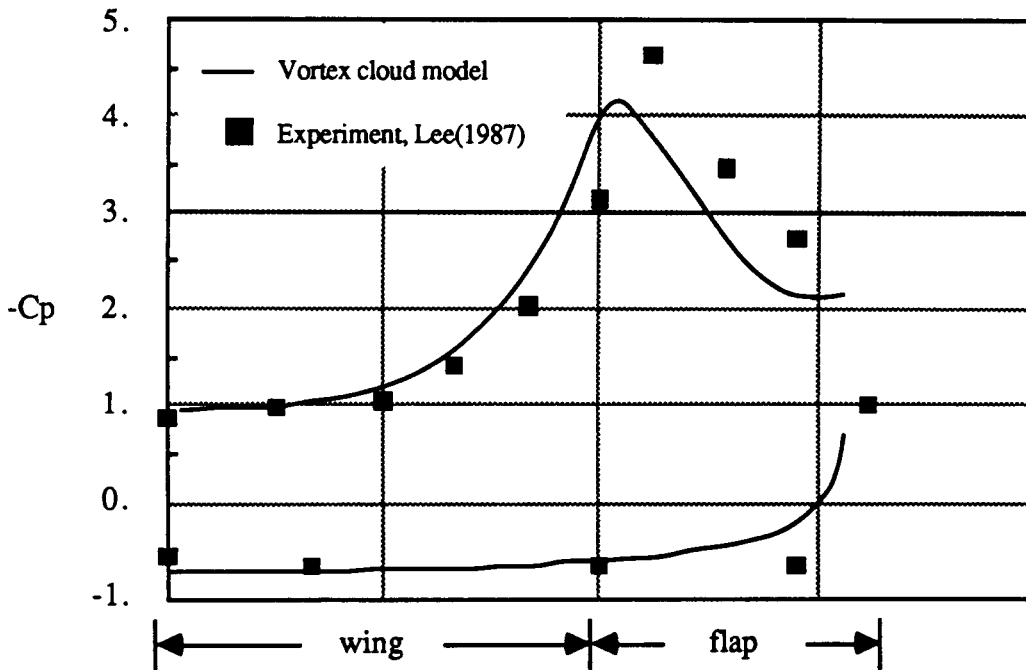
Fig. 53 Shear layer geometry and surface pressure distribution, \alpha = 35 deg., \delta = 15 deg.
