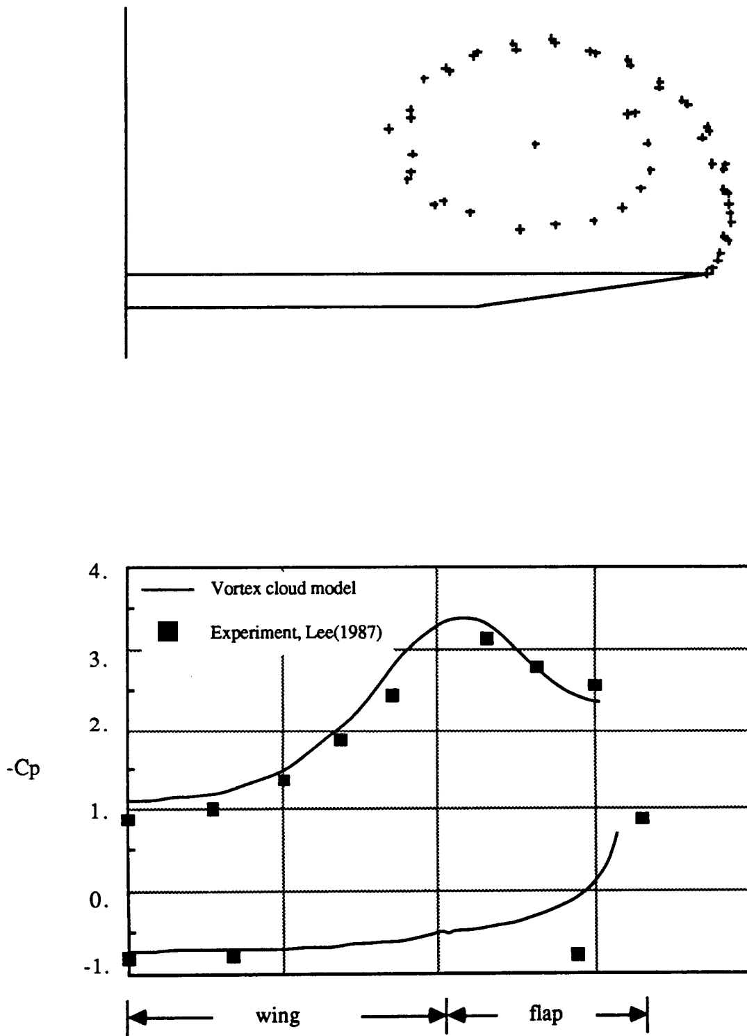
Fig. 52 Shear layer geometry and surface pressure distribution, \alpha = 35 deg., \delta = 0 deg.
