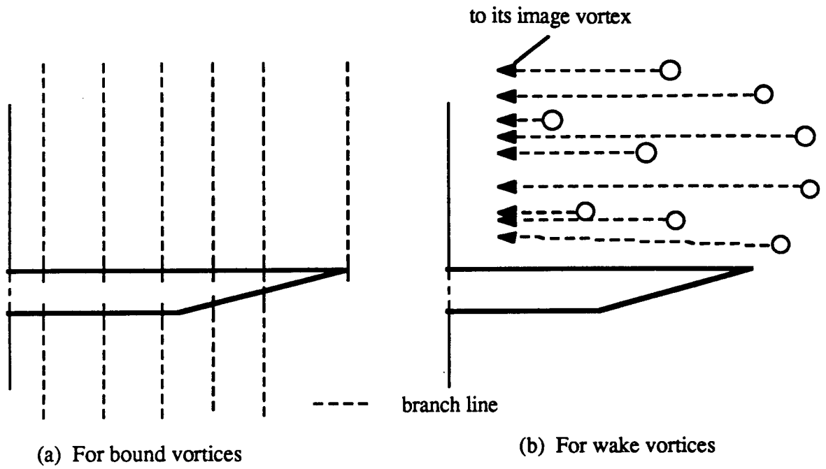
Fig. 37 Branch lines
