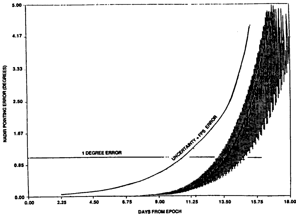
Figure 8. UARS Nadir-Pointing Error (Prediction Uncertainty Added) for a 7-Day Fit of FPS (No Residuals)
