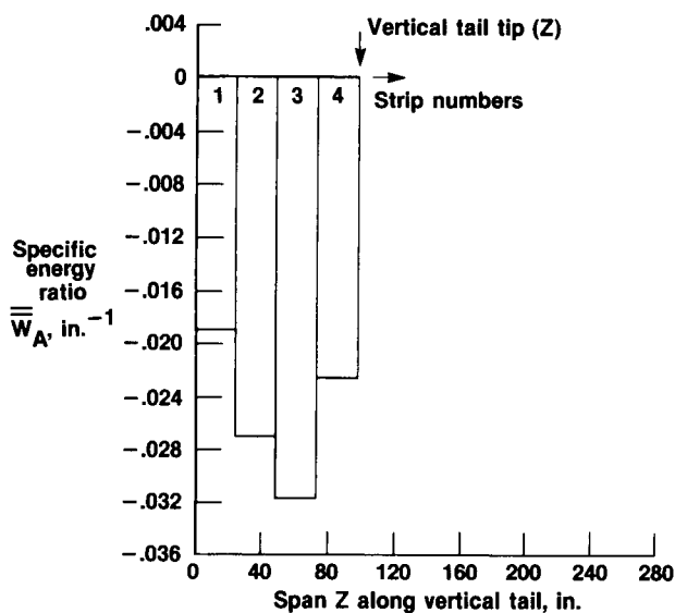
(a) Vertical tail.
