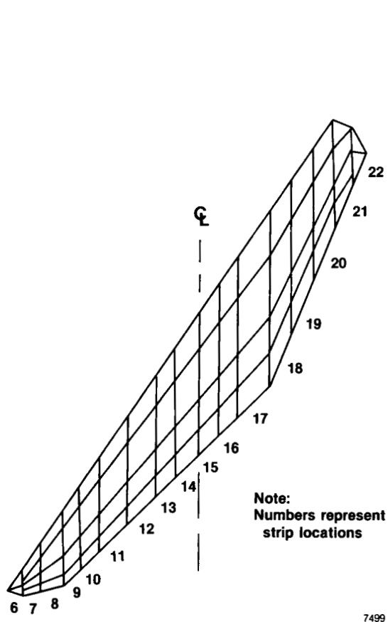
(a) Oblique wing planform skewed 65°.
