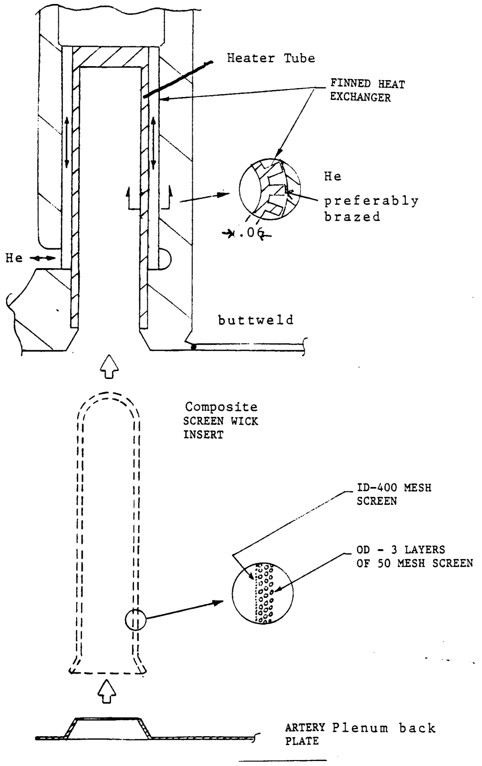
Figure 5.8 Condenser Assembly (with 10 finned tube cavities)
