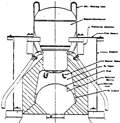
DoE/NASA Terrestrial 25 kWe Power Module MTI/Sanders/Thermacore
