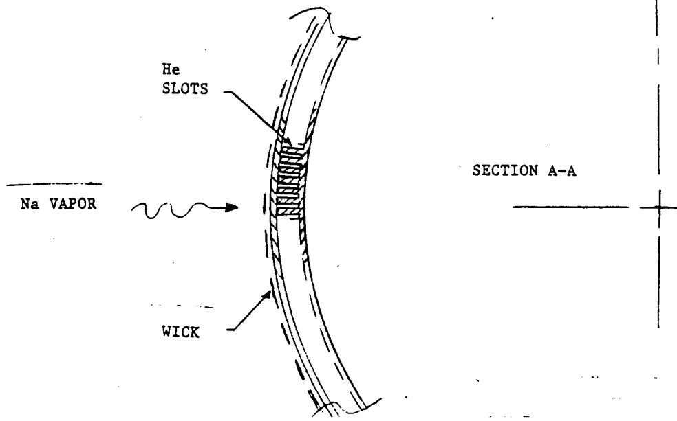
Figure 5.5 Condenser Design for Annular Heater Head Configuration
