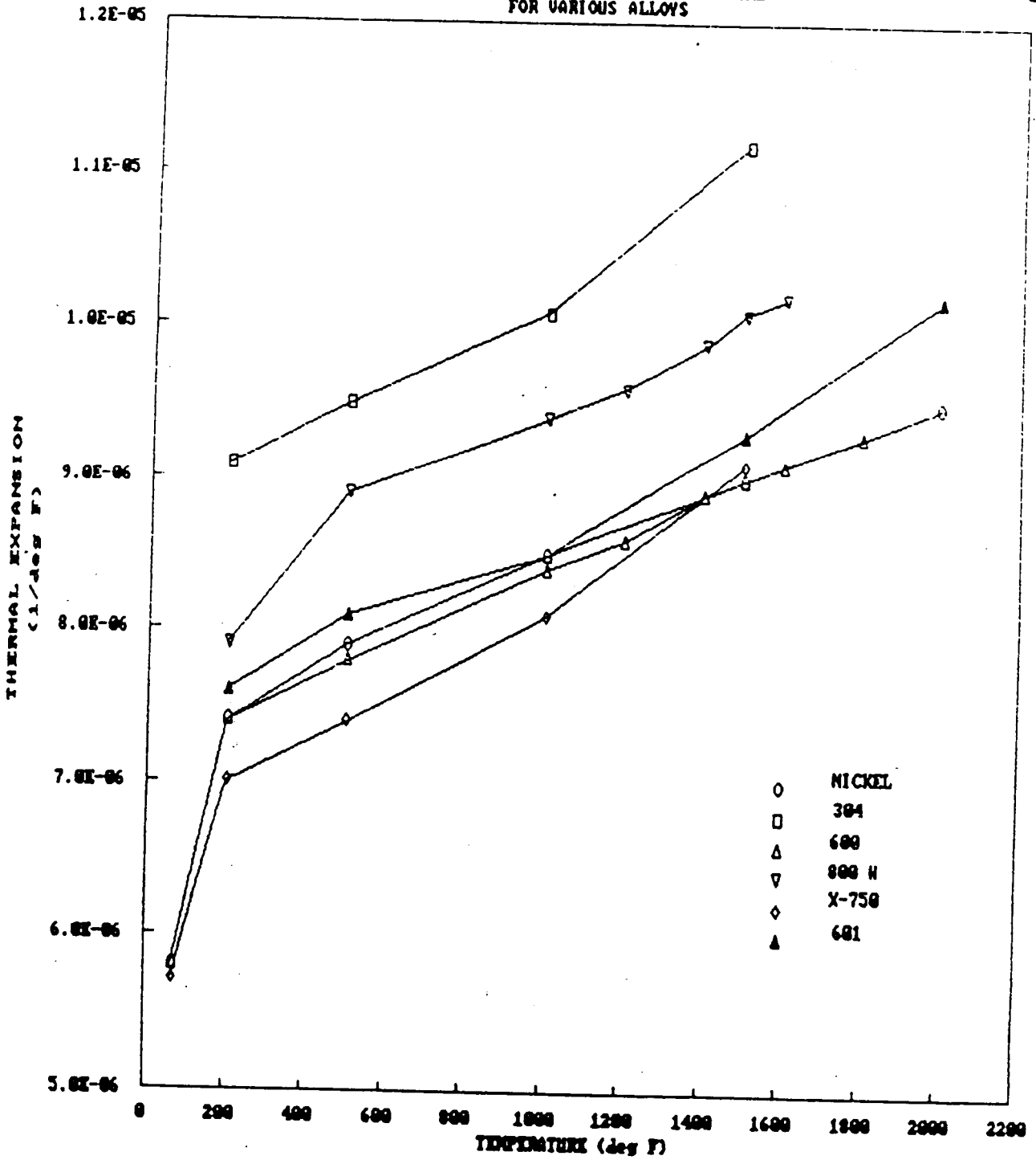
THERMAL EXPANSION VS. TEMPERATURE FOR VARIOUS ALLOYS
