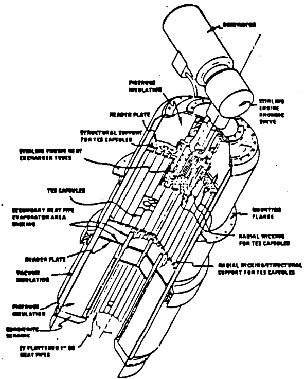
(b) JPL/GE STIRLING RECEIVER CONCEPT
