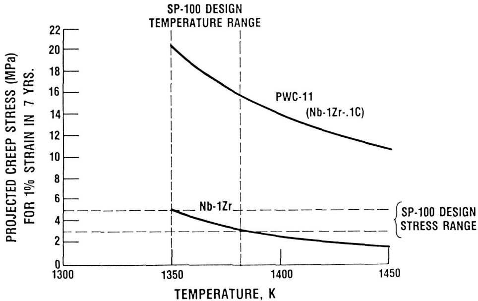
FIGURE 10. - CREEP POTENTIAL OF PWC-11 COMPARED TO Nb-1Zr.
