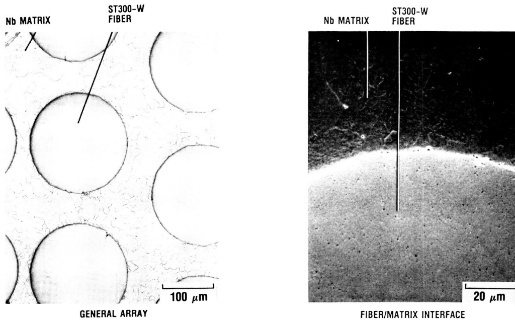
FIGURE 15. - TUNGSTEN FIBER REINFORCED NIOBIUM MATRIX COMPOSITES AS-FABRICATED MICROSTRUCTURE.
