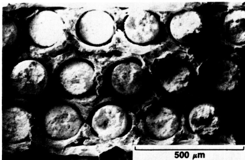
FIGURE 21. - FRACTURE SURFACE OF ST300/Nb COMPOSITE SPECIMEN.
