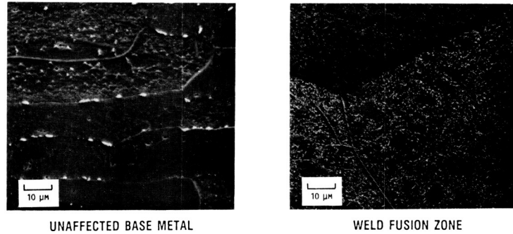
FIGURE 7. - MICROSTRUCTURES OF ELECTRON BEAM WELDED PWC-11.
