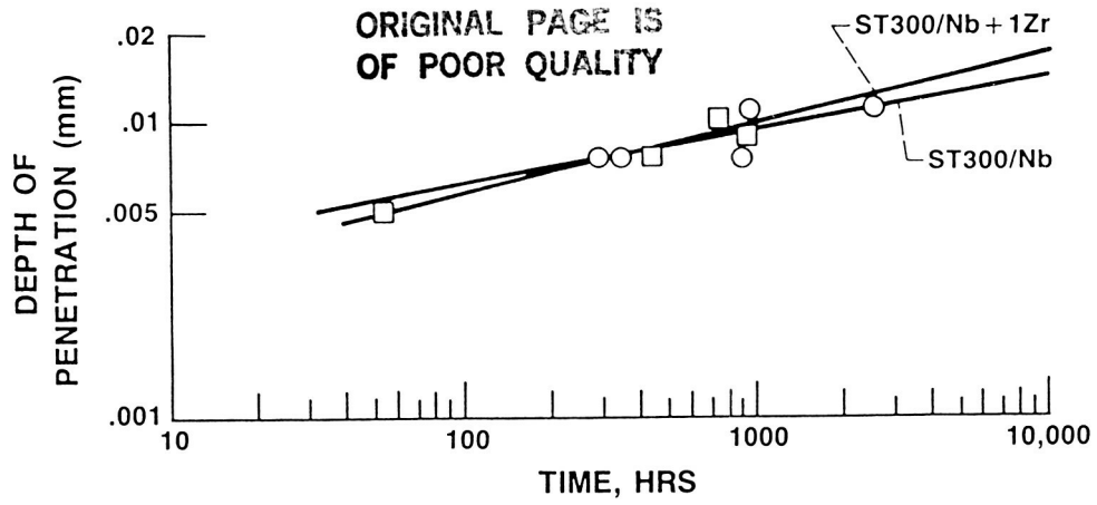
FIGURE 17. - DEPTH OF REACTION PENETRATION VERSUS TIME AT 1500 K.
