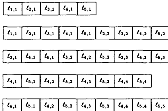
Figure 20: The organization of \ell_{i,j} 's in the working array.
