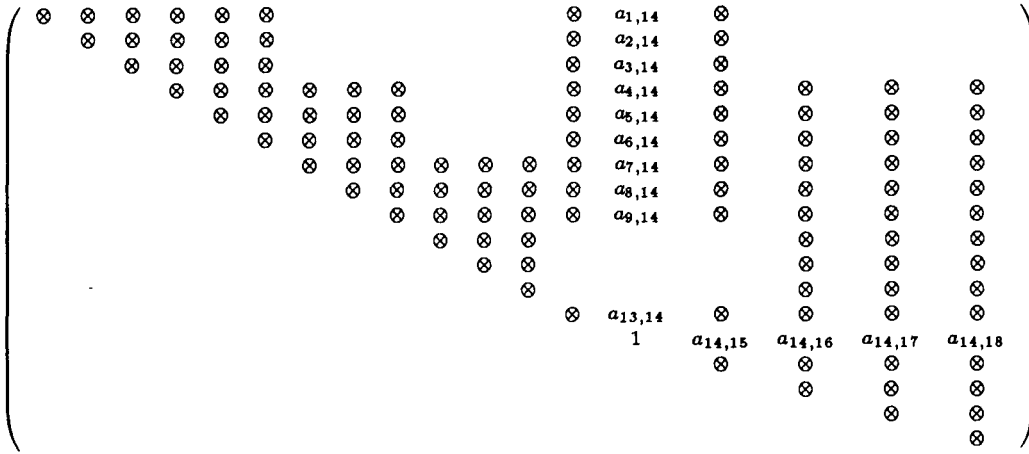
Figure 29: Nonzero entries in the upper triangle of \mathcal{K} .
