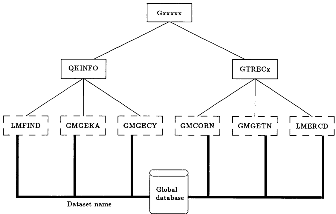
Figure 23: The coupling of CSM-interface modules and GAL-processors.
