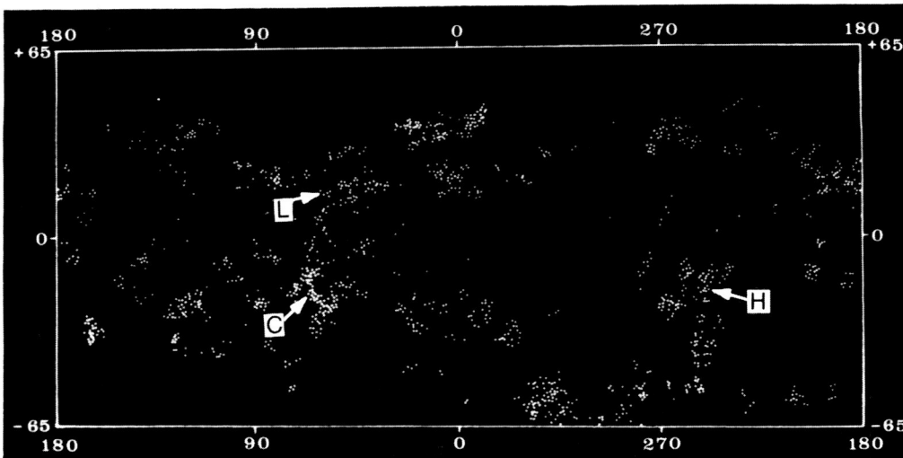
Figure 2. Map of fluidized craters on Mars (revised from Mouginis-Mark, 1979), showing the three proposed sampling sites : Coprates (C), Lunae Planum (L), and Hesperia Planum (H).
