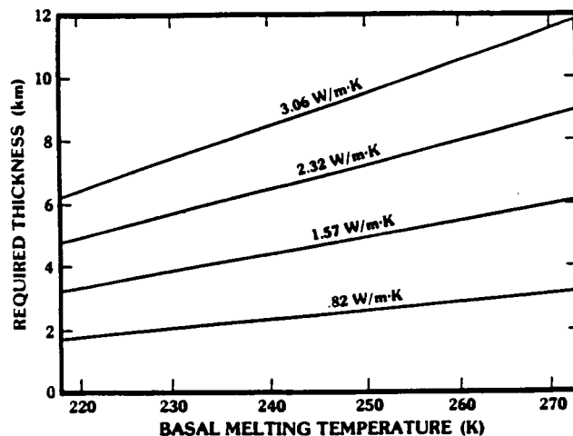
Fig. 2. Polar deposit thicknesses required for basal melting based on a mean annual surface temperature of 157 K, a geothermal heat flux of 3 \times 10^{-2} \text{ W m}^{-2} , and thermal conductivities covering the range from 0.82 to 3.06 \text{ W m}^{-1} \text{ K}^{-1} .
