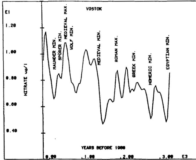
Figure 1. Smoothed curve of \text{NO}_3^- concentrations for the past 3000 years from Vostok firn core, Antarctica.
