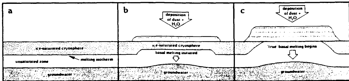
Fig. 1. An idealized cross section of the polar crust illustrating the possible time evolution of basal melting. The sequence depicts (a) a time prior to the deposition of any dust and ice, (b) the onset of deposition and basal melting, and (c) melting at the actual base of the deposits.
