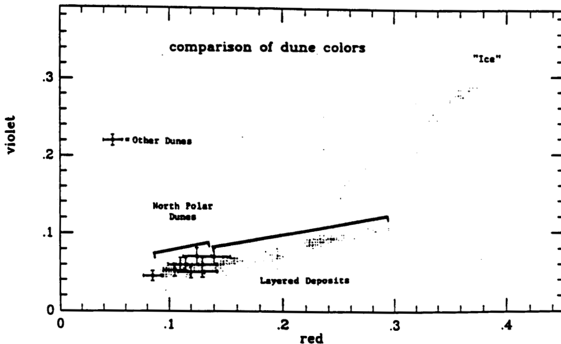
Fig. 3. Colors of polar layered deposits dunes and "ice" at -83^{\circ}\text{N} , 240^{\circ}\text{W} . Data from VO images with scattering function used to compare data from different areas. P.L.D. contain bright, red "dust," and some darker material. Dune colors from several locations at lower latitudes are compared, and are similar to polar dunes ( R/V - 2.0 ).
