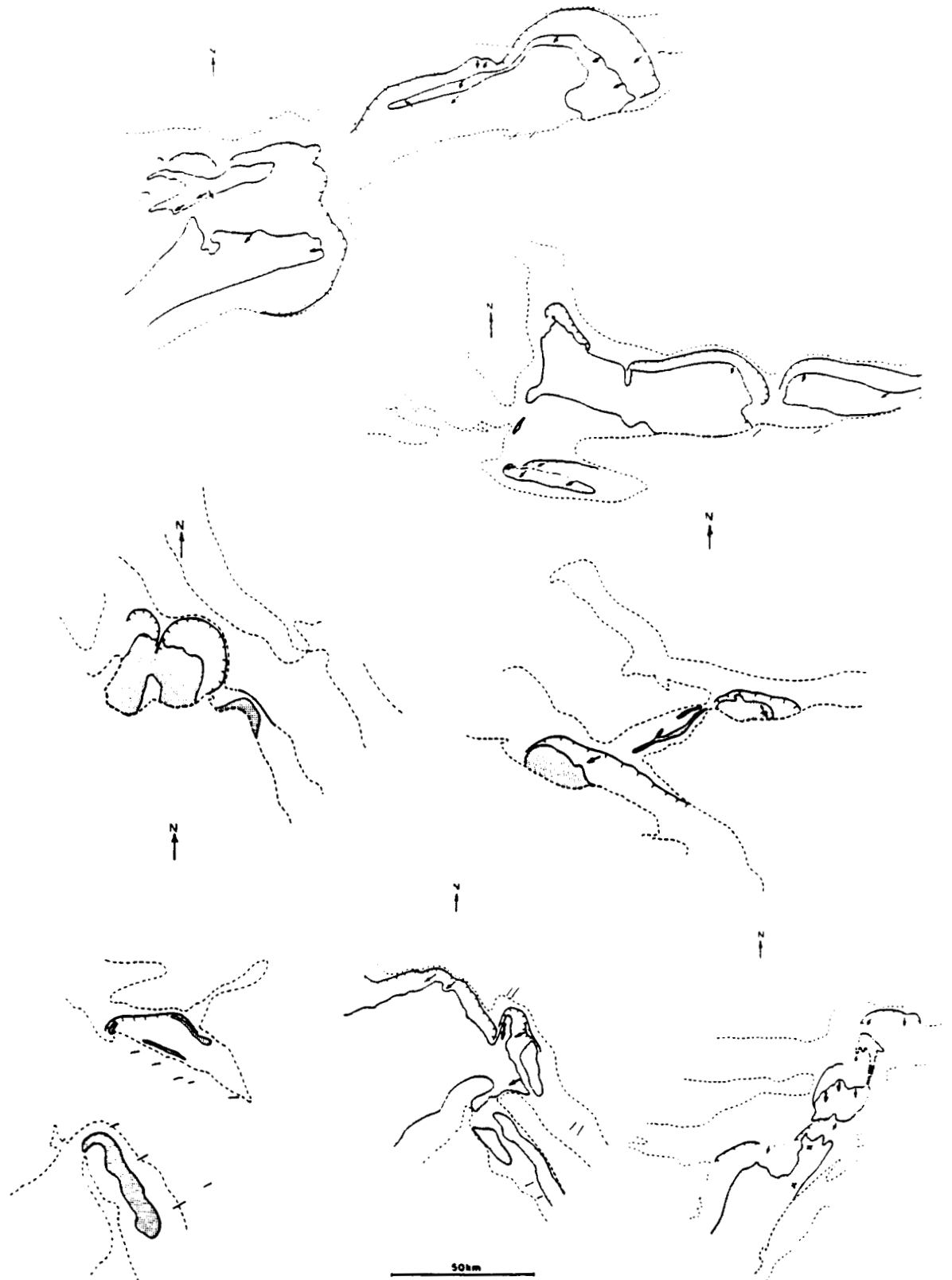
Fig. 1. Examples of the association of polar dunes and steep, arcuate scarps in P.L.D. Stippled areas are dunes, dashed lines mark trough margins, and scarps are hachured lines. Wind directions from barchan orientations, framing dunes, and wind streaks indicate flow out from the scarps.
