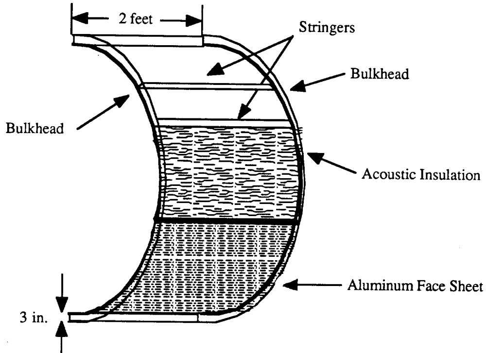
Figure 8.3 : Fuselage Cut-out
