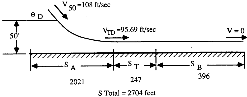
Figure 6.2 : Landing Schematic
