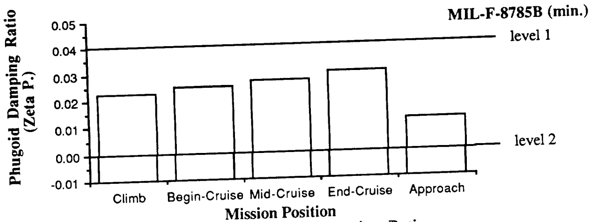
Figure 9.5 : Phugoid Damping Ratio
