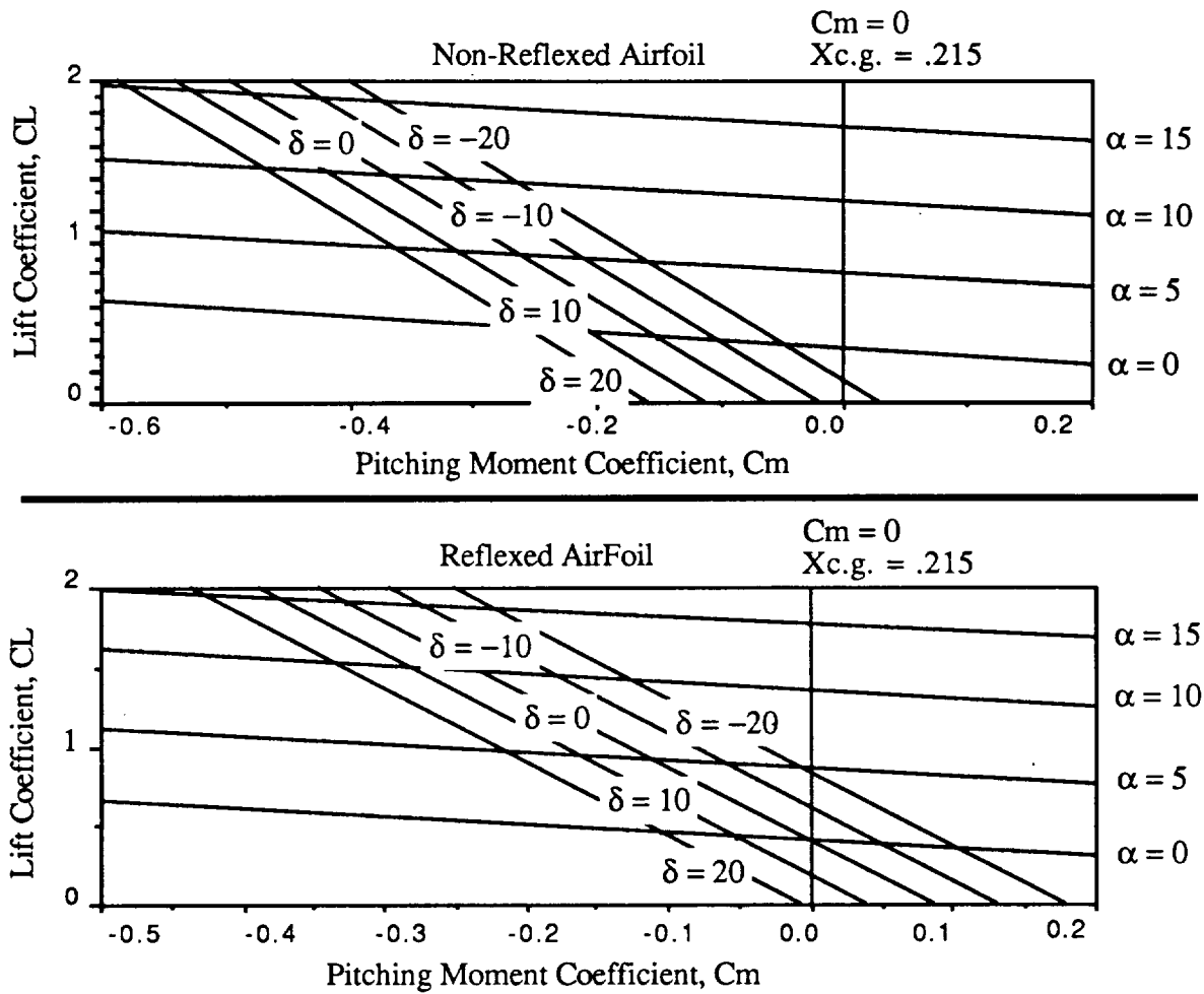
Figure 9.2 : Trim Conditions for the CONDOR
