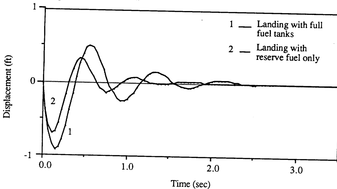
Figure 8.11 : Landing Gear Time Response
