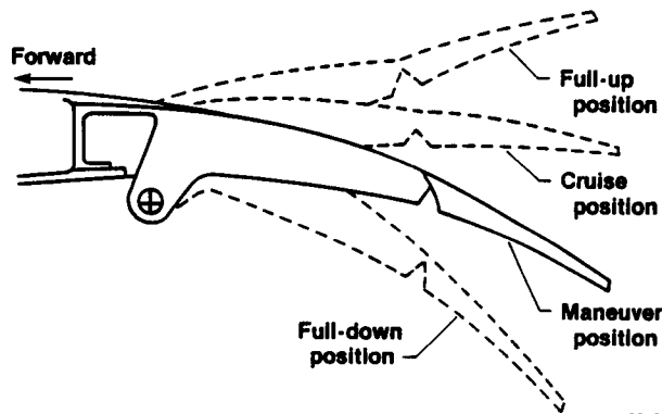
Figure 14. X-29A full-span flap geometry.
