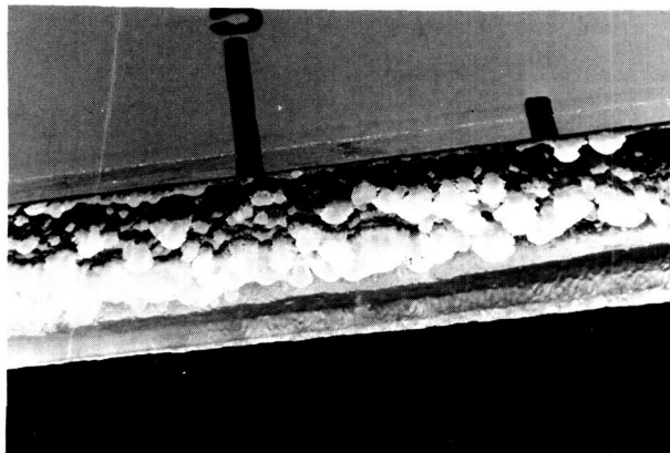
FIGURE 13. - CLOSE-UP DETAIL OF ICE FEATHERS AND PRIMARY FORMATION. 2100 RPM, \tau = 3.6\text{ MIN} , 15\text{ }\mu\text{m} , 31.3\text{ M/S} , -12.2\text{ }^{\circ}\text{C} , .5\text{ g/M}^3 , \theta_{75} = 4^{\circ} .
