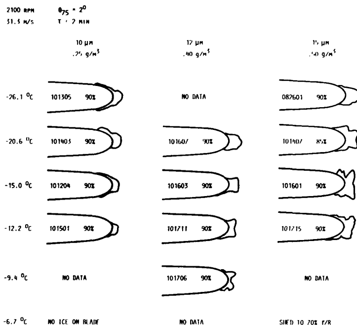
FIGURE 9. - TEMPERATURE EFFECT ON ICE ACCRETION.
