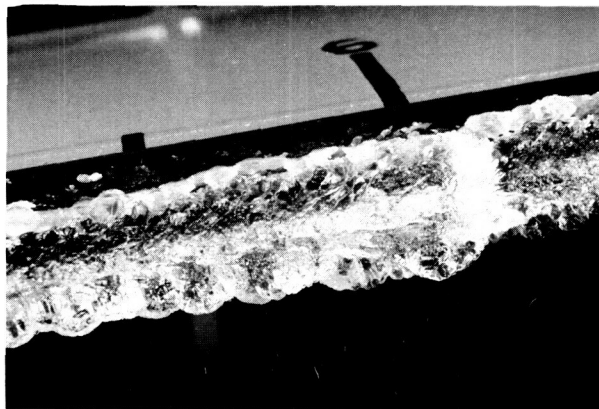
FIGURE 14. - CLOSE-UP DETAIL OF LEADING EDGE ICE FORMATION. 2100 RPM, \tau = 5.4\text{ MIN} , 15\text{ }\mu\text{m} , 31.3\text{ M/S} , -9.4\text{ }^{\circ}\text{C} , .5\text{ g/M}^3 , \theta_{75} = 4^{\circ} .
