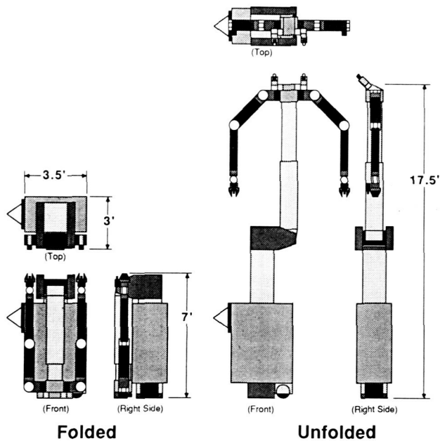
Figure 1. FTS Dimensions
