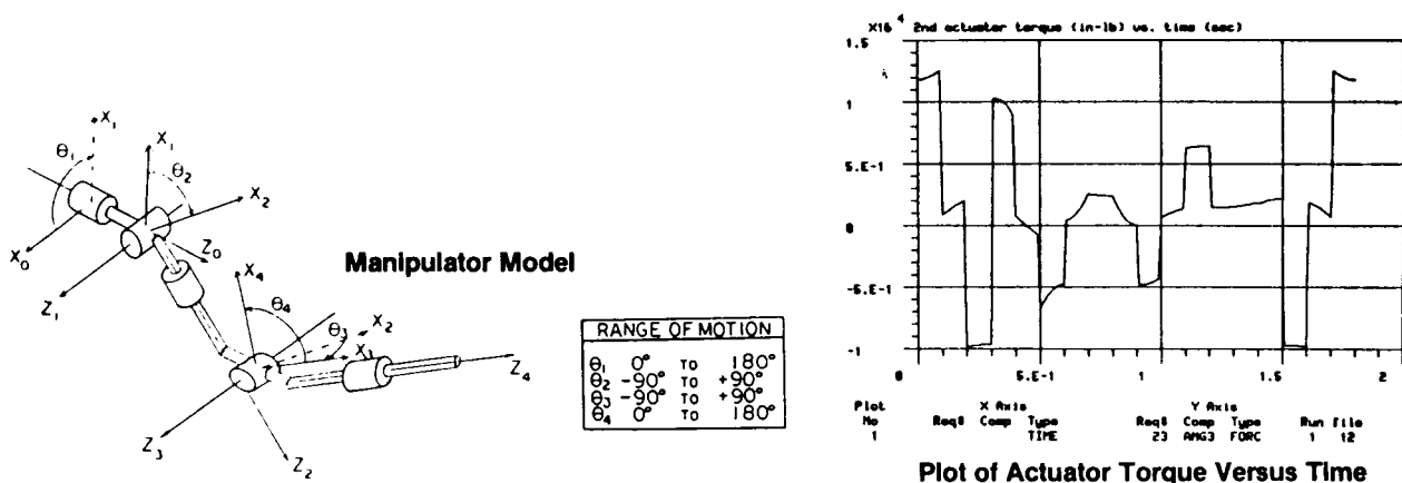
Figure 7. Analysis of Manipulator Dynamics
