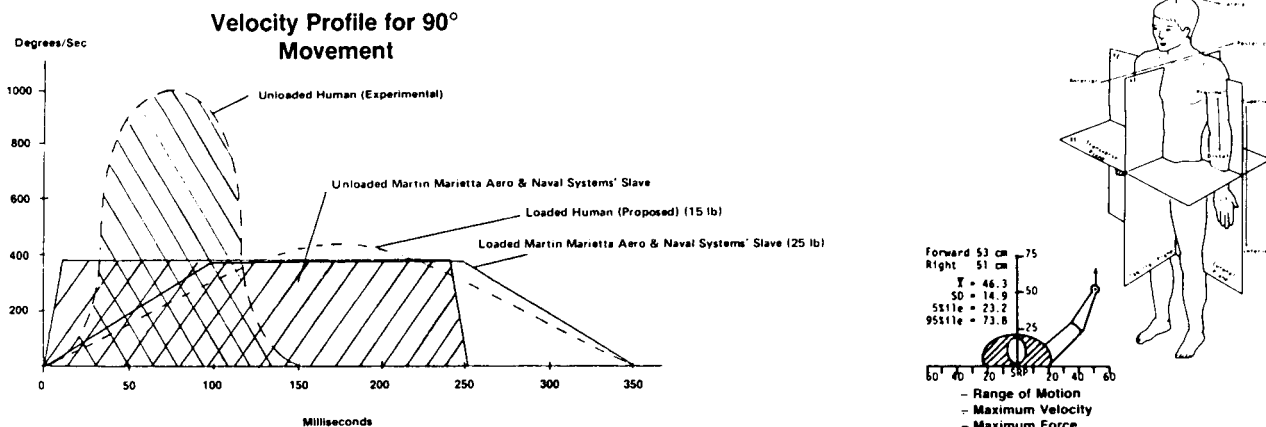
Figure 6. Human Performance Characteristics
