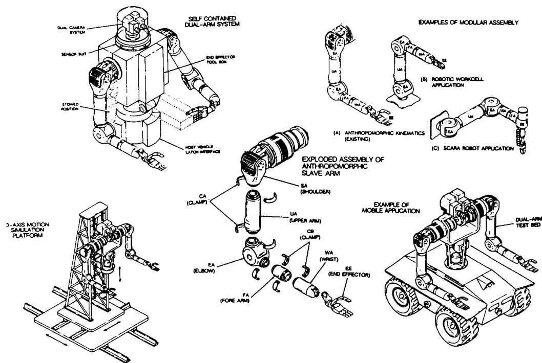
Figure 9. Anthropomorphic Manipulator
