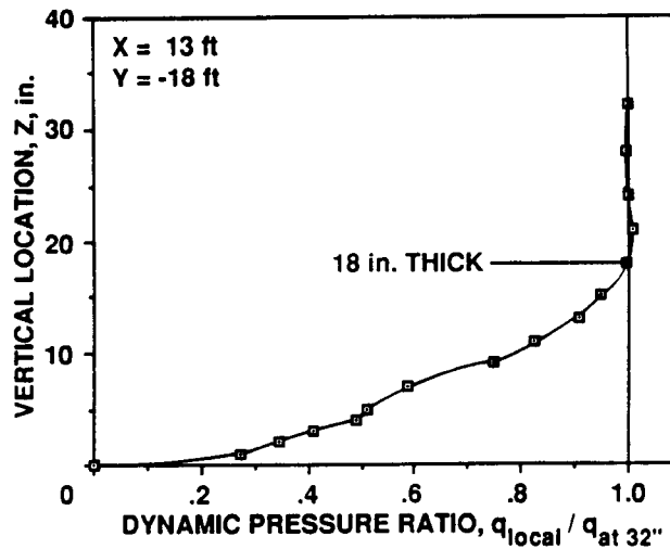
Figure 59.— Dynamic pressure profiles from the fixed rakes on the test section floor.
