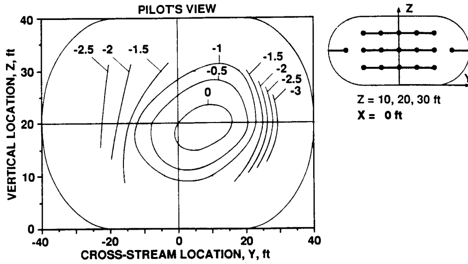
Figure 43.— Total pressure contour plot (lines of equal (p_t - p_{t,cl}) at U_{ts} = 300 knots, 10% air exchange)).
