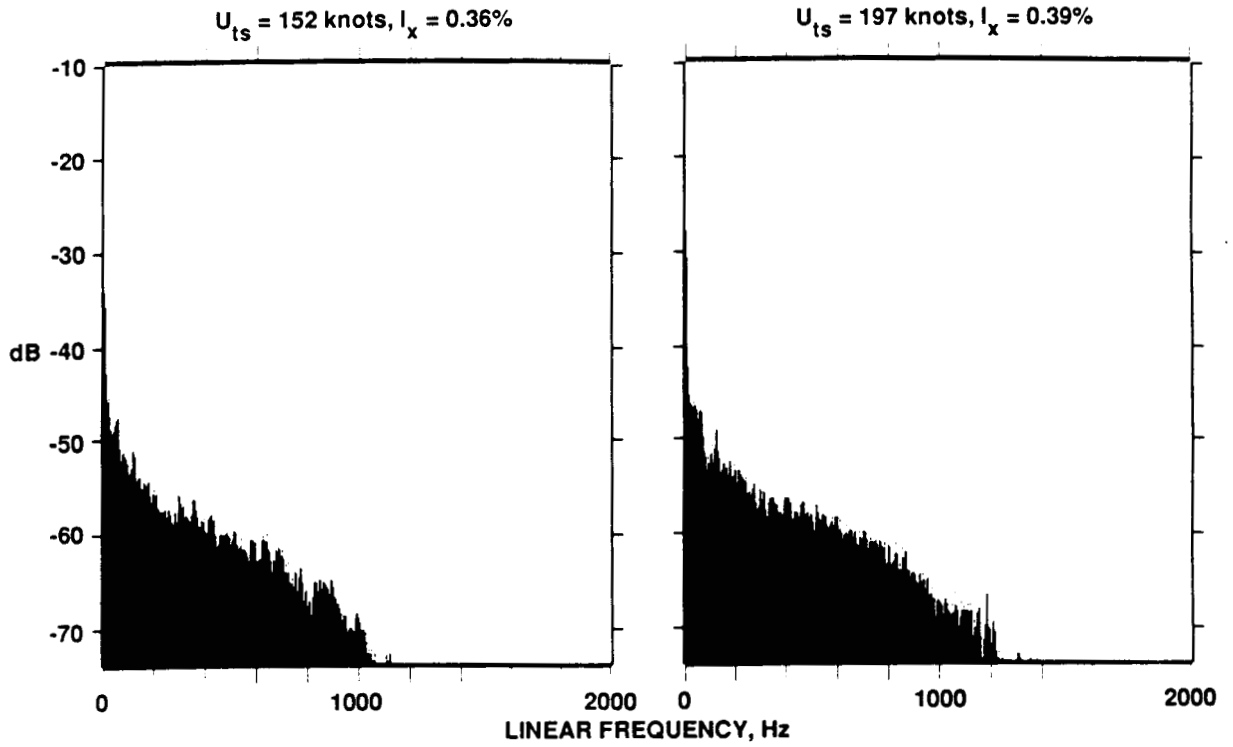
Figure 66.— Energy spectra ( U_{ts} = 152 and 197 knots).
