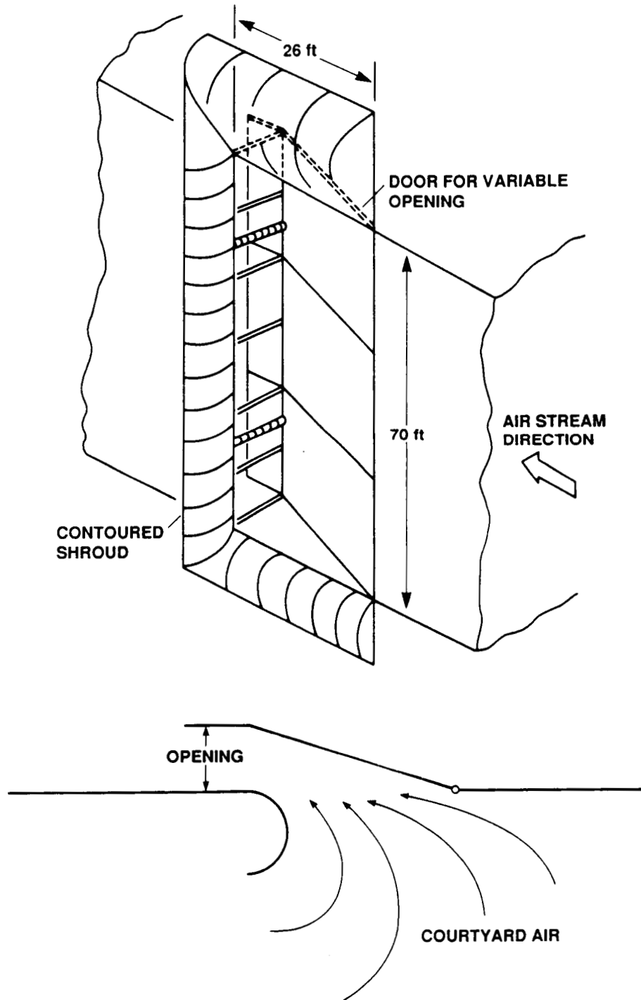
Figure 7.- Wind tunnel air-exchange system inlet.
