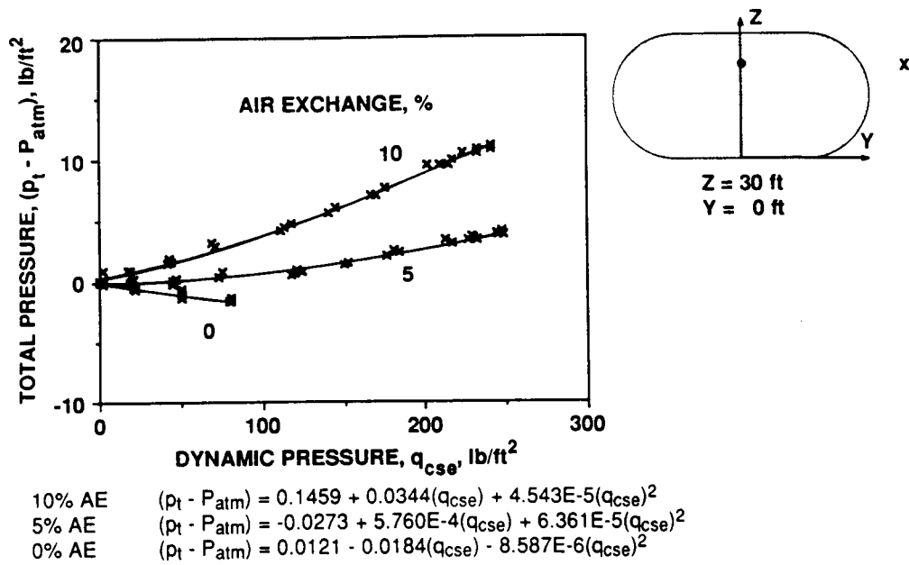
Figure 38.— Indicated total pressure on centerline versus scale dynamic pressure (Z = 30 ft).
