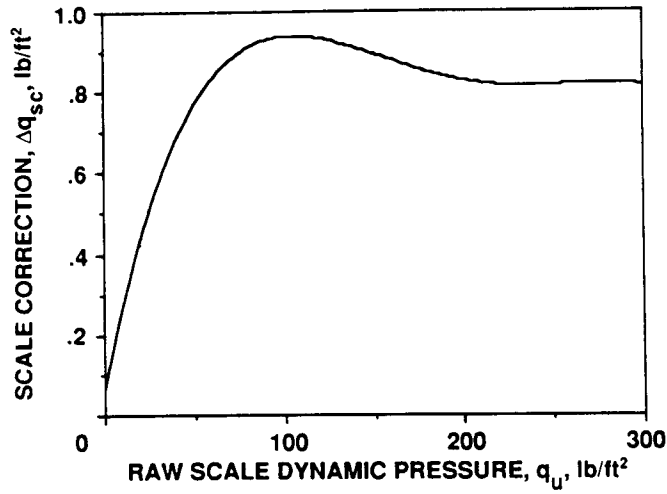
Figure 17.— Dynamic pressure scale correction versus scale dynamic pressure.
