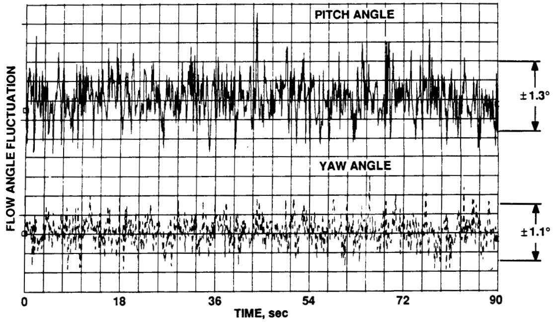
Figure 68.— 90 sec pitch and yaw angle time history for Y = 20 ft station ( U_{ts} = 300 knots).
