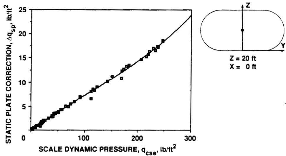
Figure 20.— Dynamic pressure static plate correction versus scale dynamic pressure.
