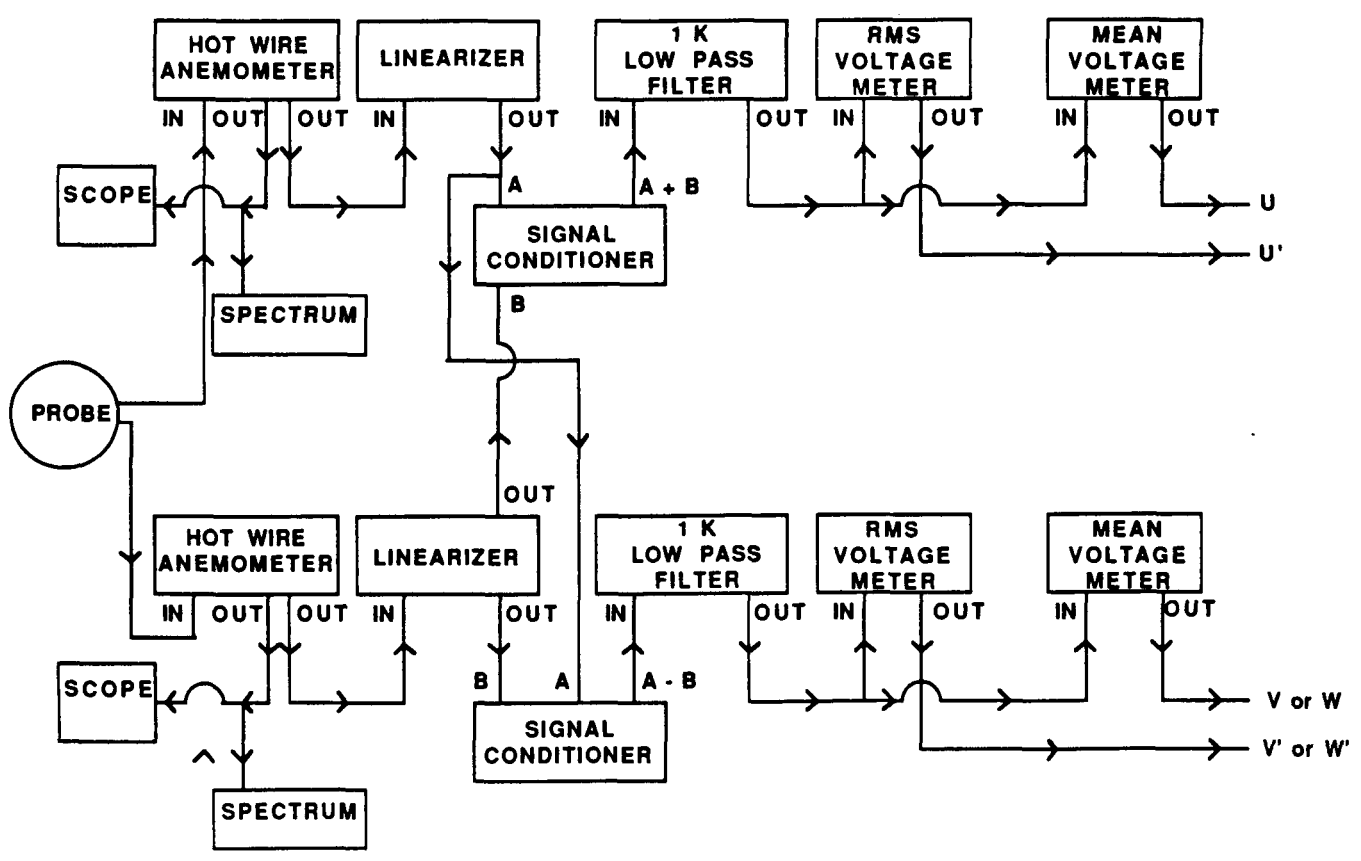
Figure 61.— Hot wire anemometer instrumentation diagrams.
