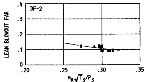
(G) LEAN BLOWOUT CHARACTERISTICS.
