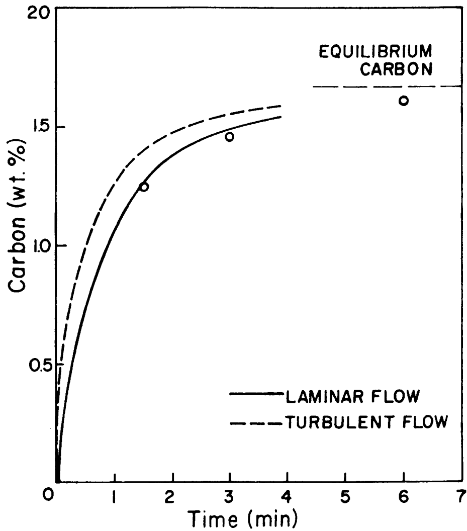
Fig. 3 — Experimental carburization results (CO 2.15/CO 2 at 38.9 atm and 1650 °C) ■ compared with the theoretical predictions for turbulent and laminar flow in the levitated drop.
