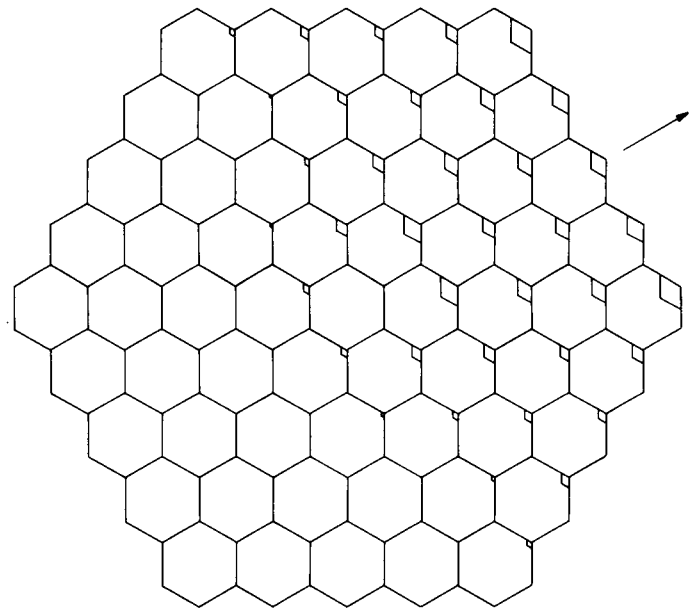
Fig. 2. Partial shutters as viewed along the length of the integral sunshade tubes, when the projected Sun vector (arrow) is directed parallel to the line joining the hexagon corners from lower left to upper right. This figure shows shading necessary for E = 9 degrees.
