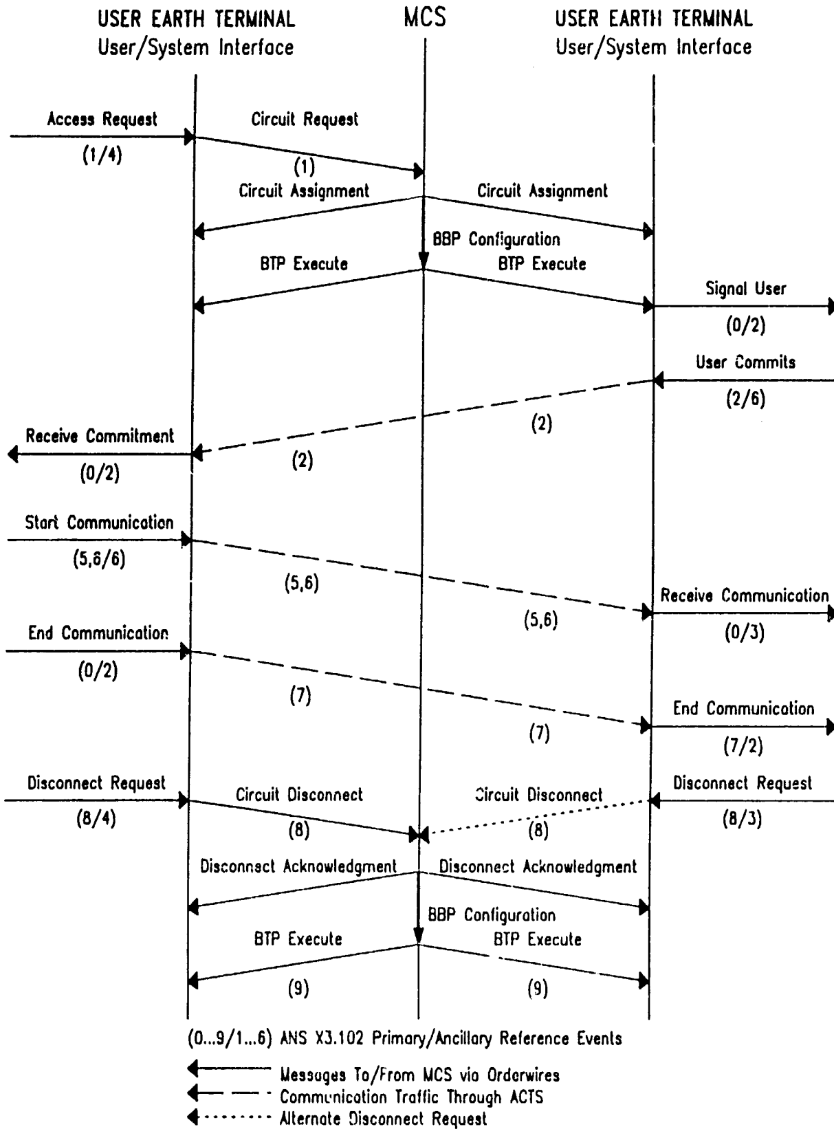
Figure 10. Typical ACTS LBR system communication session.
