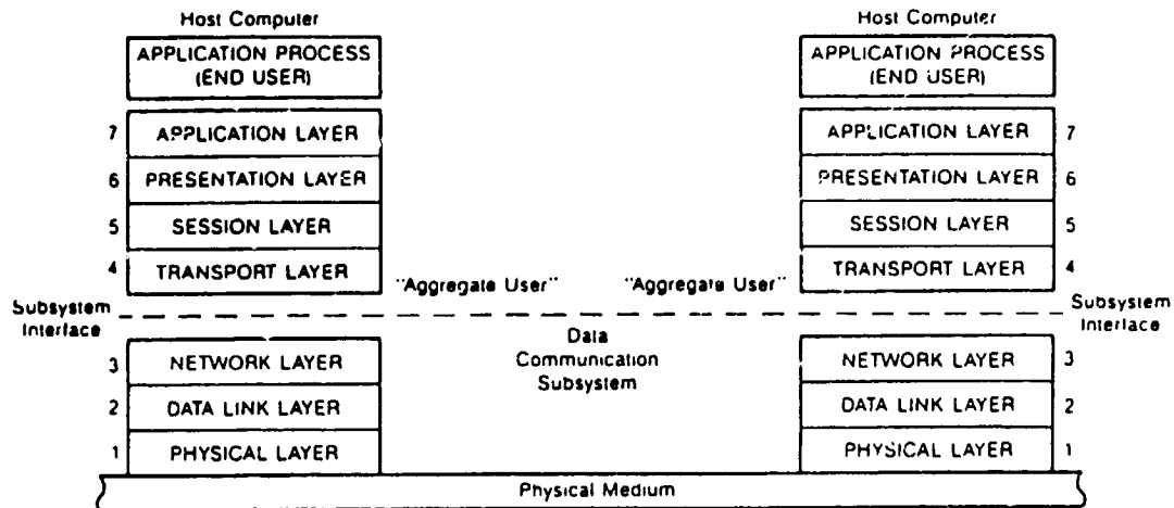
(b) Protocol Layer Boundaries Delimiting a Subsystem
