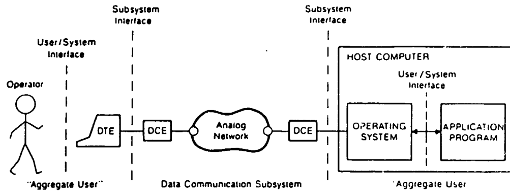
(a) DTE/DCE Interfaces Delimiting a Subsystem
