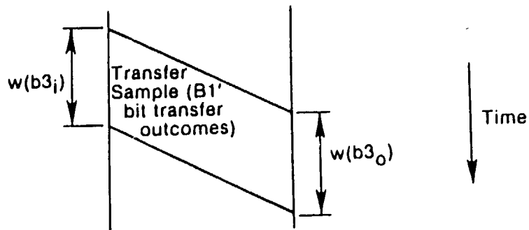
Case 1. No rate conversion : w(b3_i) = w(b3_o)
