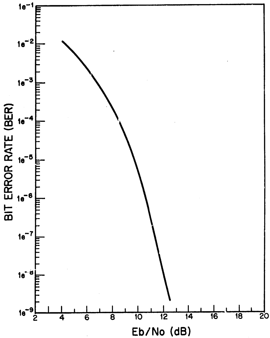
Figure A-1. Bit error rate vs. E_b/N_0 .
