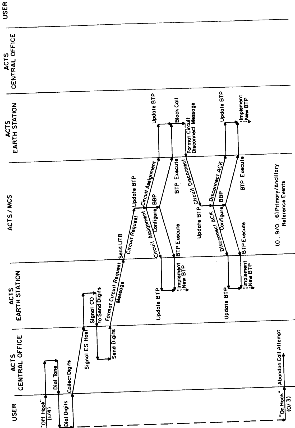
Figure 15. Unsuccessful access, blocked by destination earth station.
