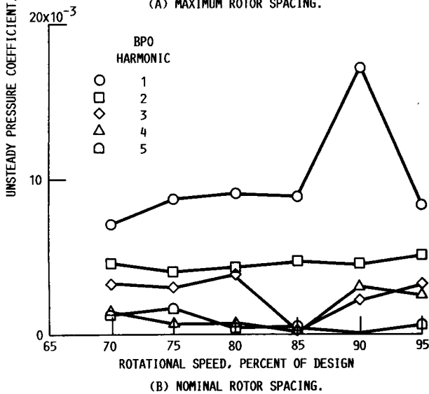
FIGURE 8. - EFFECT OF ROTOR SPEED ON BLADE PASSING ORDER AND ITS HARMONICS FOR AFT ROTOR BLADE (A3), PRESSURE SURFACE.
