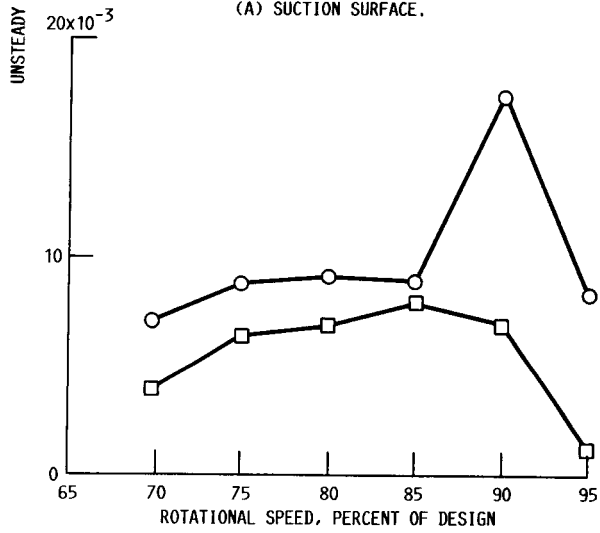
FIGURE 10. - EFFECT OF ROTOR SPACING ON BLADE PASSING ORDER TONE FOR AFT ROTOR BLADE (A3).
