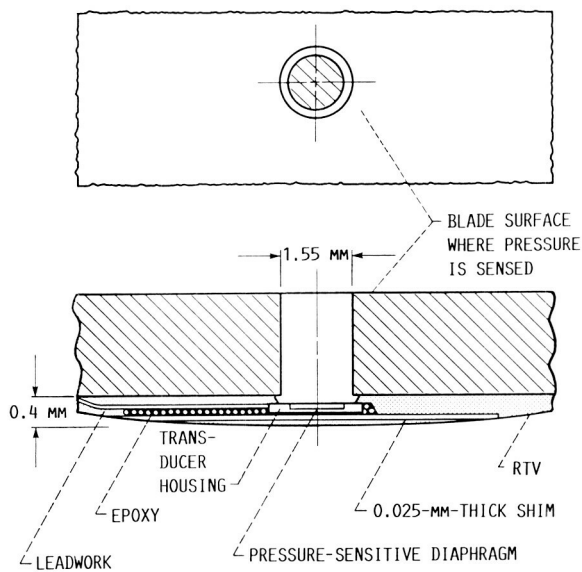
(B) TYPICAL INSTALLATION OF BLADE-MOUNTED PRESSURE TRANSDUCER SENSING THROUGH BLADE.
