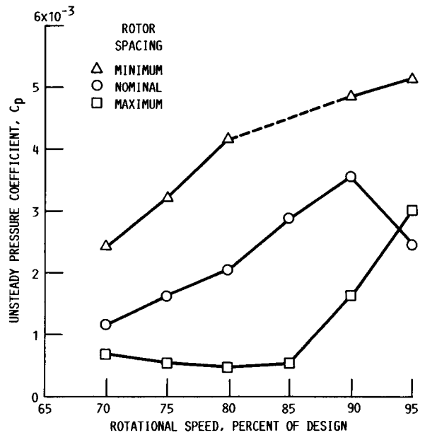
FIGURE 9. - EFFECT OF ROTOR SPACING ON BLADE PASSING ORDER TONE FOR FORWARD ROTOR BLADE (F7), SUCTION SURFACE.
