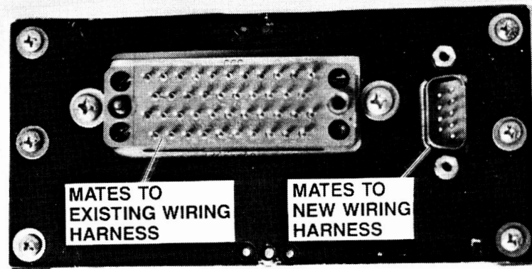
Figure C-8. Backside of interface unit.
