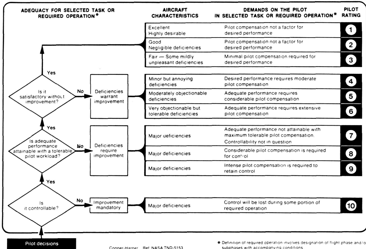
Figure 10.— The Handling-Qualities Rating Scale.
