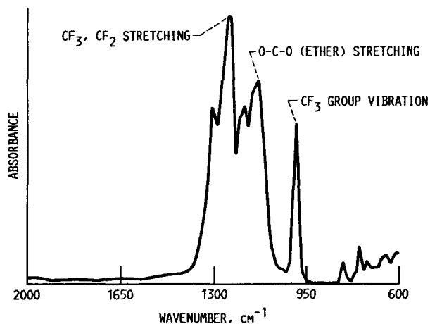
Figure 11.—FTIR spectrum of TCF-soluble matter formed from Krytox 16256.
