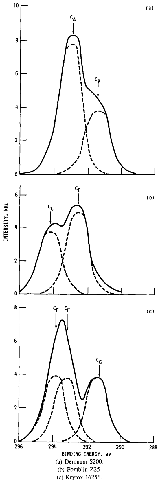
Figure 2.—C 1s XPS spectra. Substrate, 440C stainless steel.
