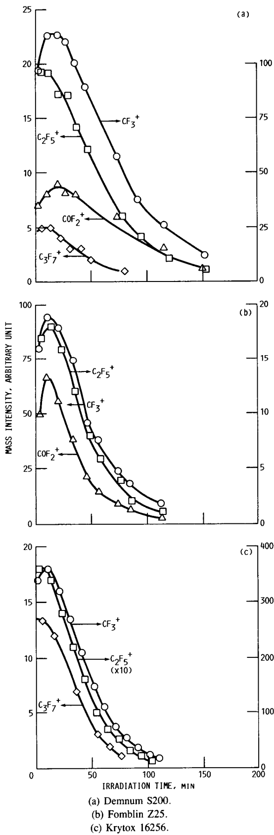
Figure 9.—Time dependence of mass intensity. Substrate, 440C stainless steel.
