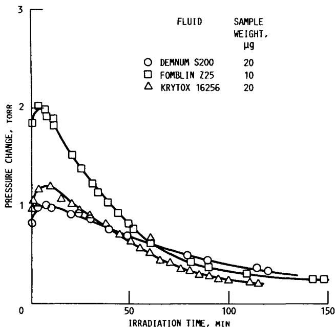
Figure 6.—Pressure change owing to gas evolution.
