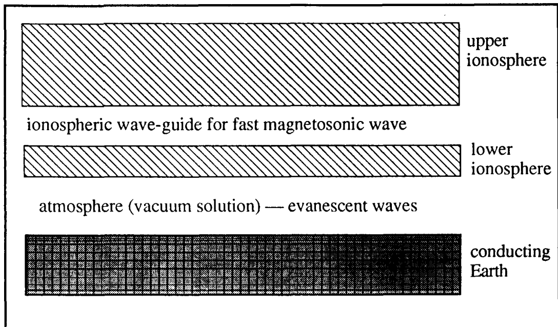
Figure 4.3. The ionospheric wave-guide and other layers of the medium
