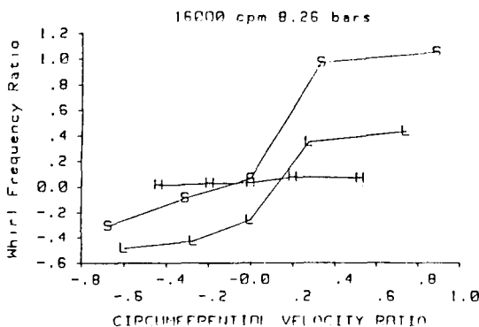
Figure 20. Whirl frequency ratio versus u_{\theta o} for smooth, labyrinth, and honeycomb seals.
